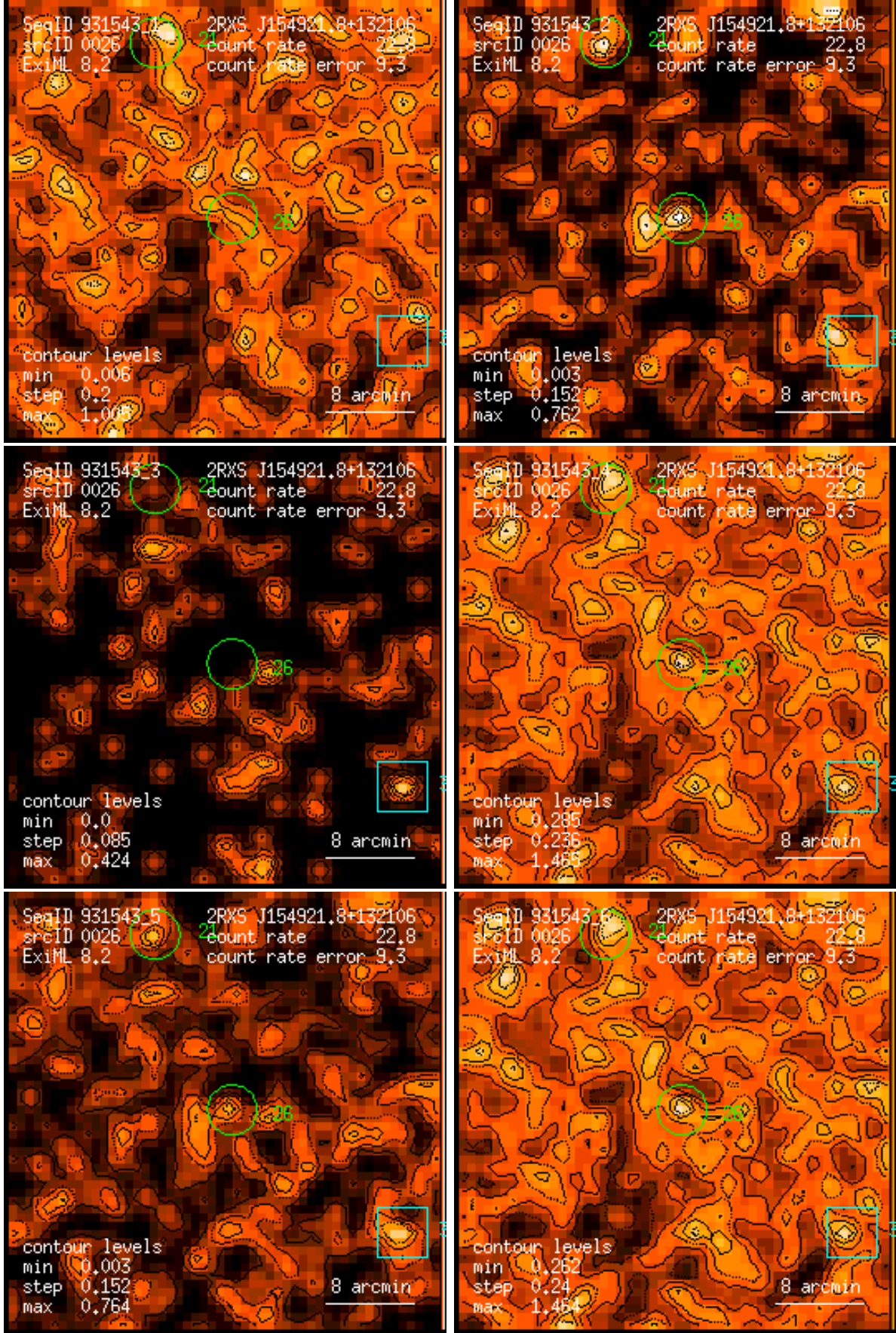
Figure 26: RASS 931543: detection 0026: band rate images, Gaussian filter: (1) PSPC channels 11 – 41, (2) 52 – 90, (3) 91 – 201, (4) 11 – 235, (5) 52 – 201, (6) 11 – 201. Broad band rates in counts/ks. Band rate contour levels in counts/ks/arcmin 2 .
