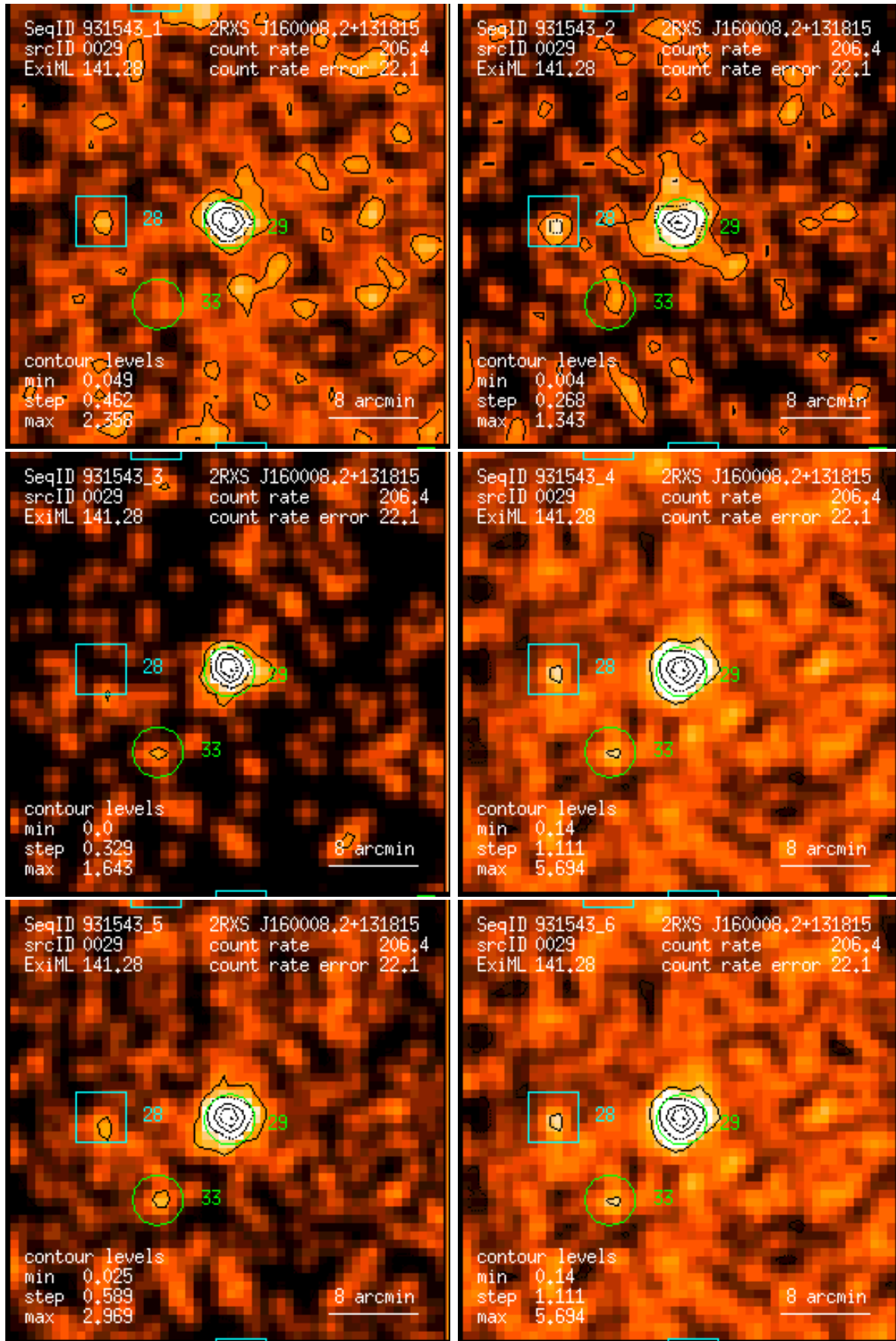
Figure 29: RASS 931543: detection 0029: band rate images, Gaussian filter: (1) PSPC channels 11 – 41, (2) 52 – 90, (3) 91 – 201, (4) 11 – 235, (5) 52 – 201, (6) 11 – 201. Broad band rates in counts/ks. Band rate contour levels in counts/ks/arcmin 2 .
