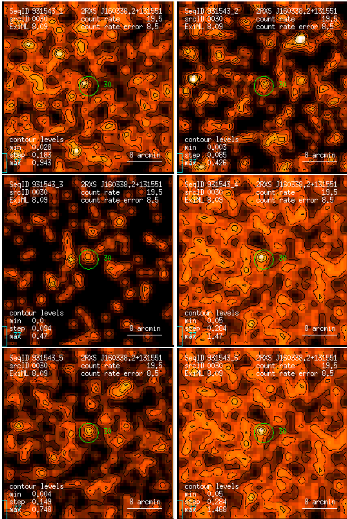
Figure 30: RASS 931543: detection 0030: band rate images, Gaussian filter: (1) PSPC channels 11 – 41, (2) 52 – 90, (3) 91 – 201, (4) 11 – 235, (5) 52 – 201, (6) 11 – 201. Broad band rates in counts/ks. Band rate contour levels in counts/ks/arcmin 2 .
