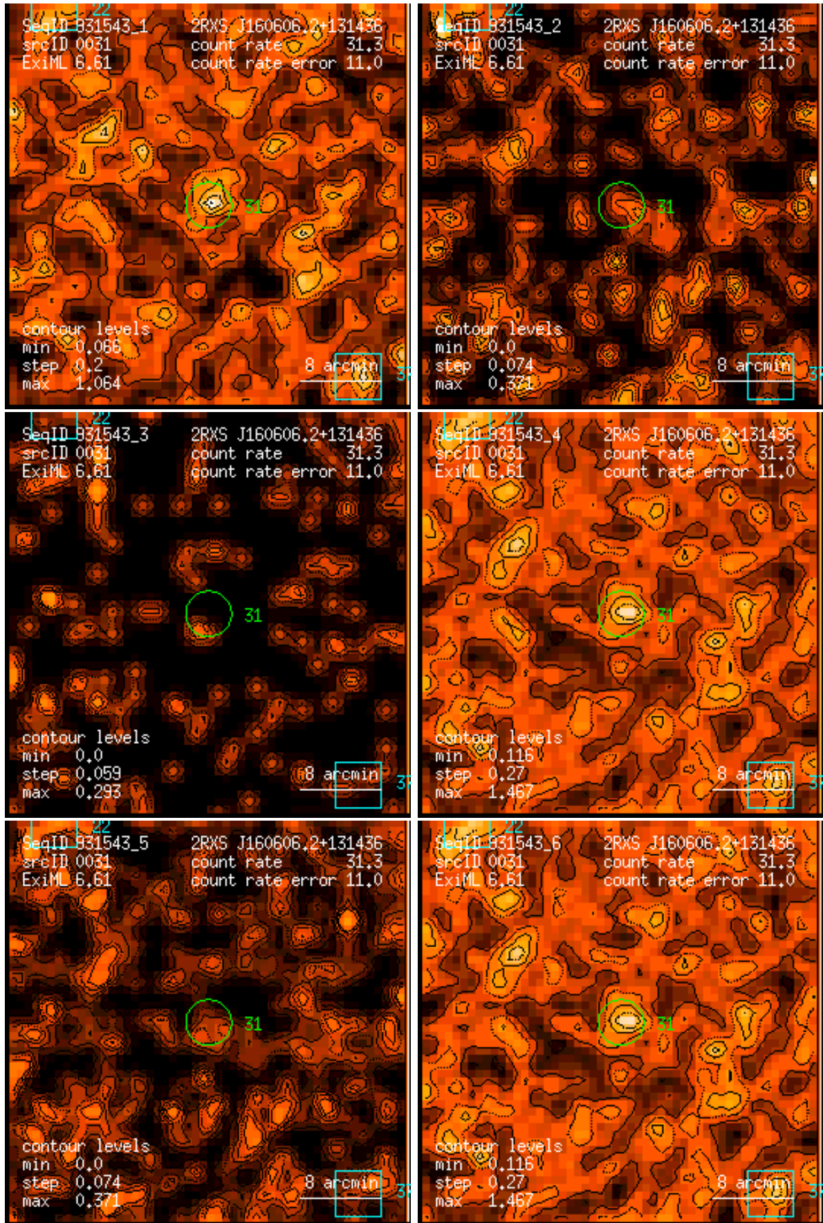
Figure 31: RASS 931543: detection 0031: band rate images, Gaussian filter: (1) PSPC channels 11 – 41, (2) 52 – 90, (3) 91 – 201, (4) 11 – 235, (5) 52 – 201, (6) 11 – 201. Broad band rates in counts/ks. Band rate contour levels in counts/ks/arcmin 2 .
