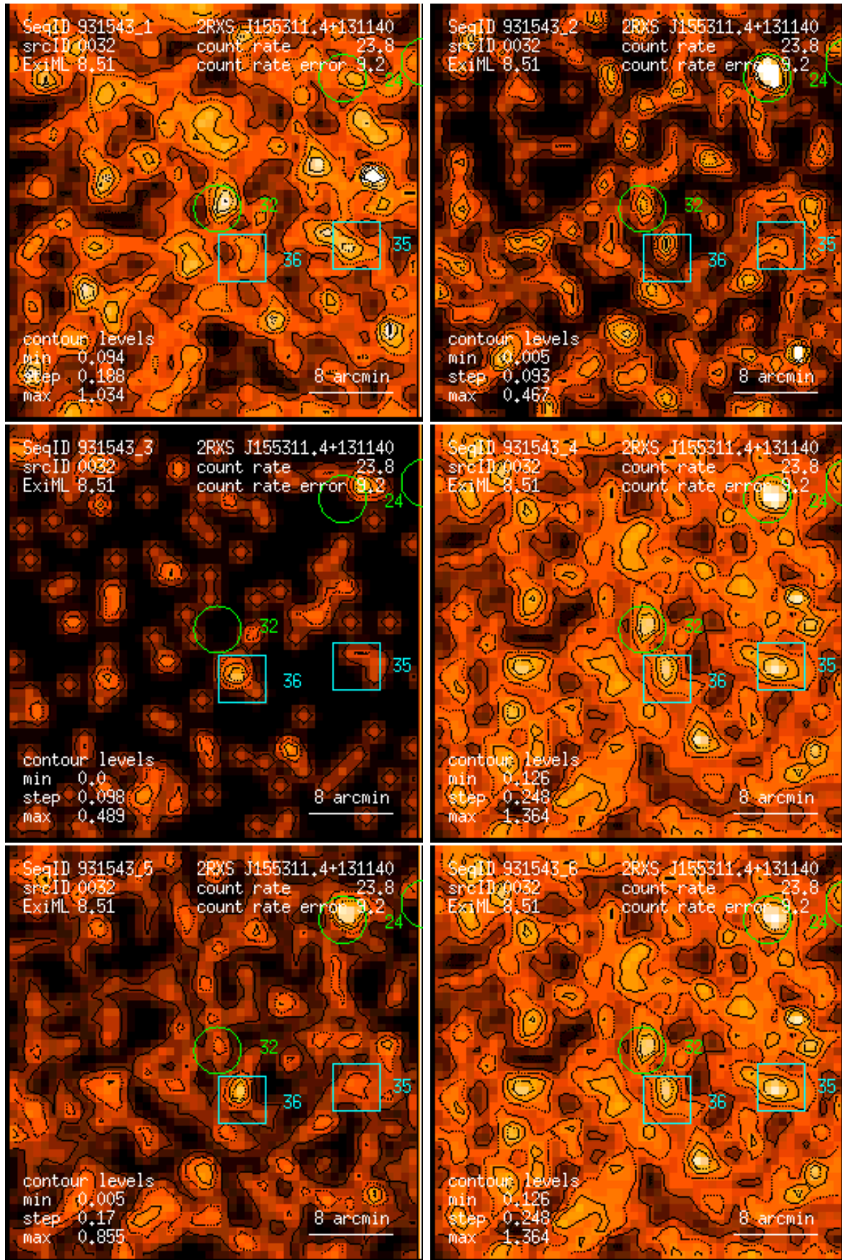
Figure 32: RASS 931543: detection 0032: band rate images, Gaussian filter: (1) PSPC channels 11 – 41, (2) 52 – 90, (3) 91 – 201, (4) 11 – 235, (5) 52 – 201, (6) 11 – 201. Broad band rates in counts/ks. Band rate contour levels in counts/ks/arcmin 2 .
