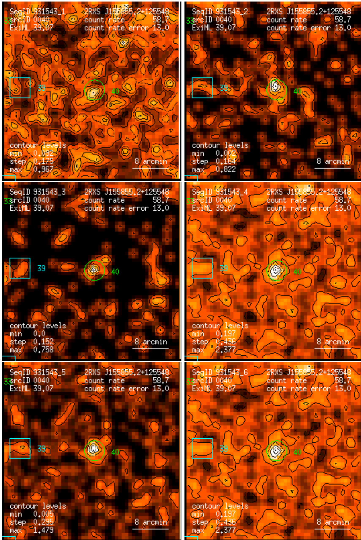
Figure 40: RASS 931543: detection 0040: band rate images, Gaussian filter: (1) PSPC channels 11 – 41, (2) 52 – 90, (3) 91 – 201, (4) 11 – 235, (5) 52 – 201, (6) 11 – 201. Broad band rates in counts/ks. Band rate contour levels in counts/ks/arcmin 2 .
