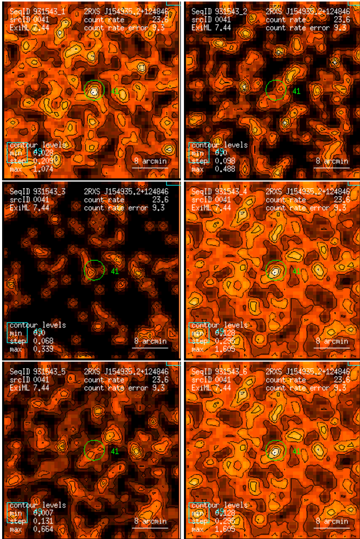
Figure 41: RASS 931543: detection 0041: band rate images, Gaussian filter: (1) PSPC channels 11 – 41, (2) 52 – 90, (3) 91 – 201, (4) 11 – 235, (5) 52 – 201, (6) 11 – 201. Broad band rates in counts/ks. Band rate contour levels in counts/ks/arcmin 2 .
