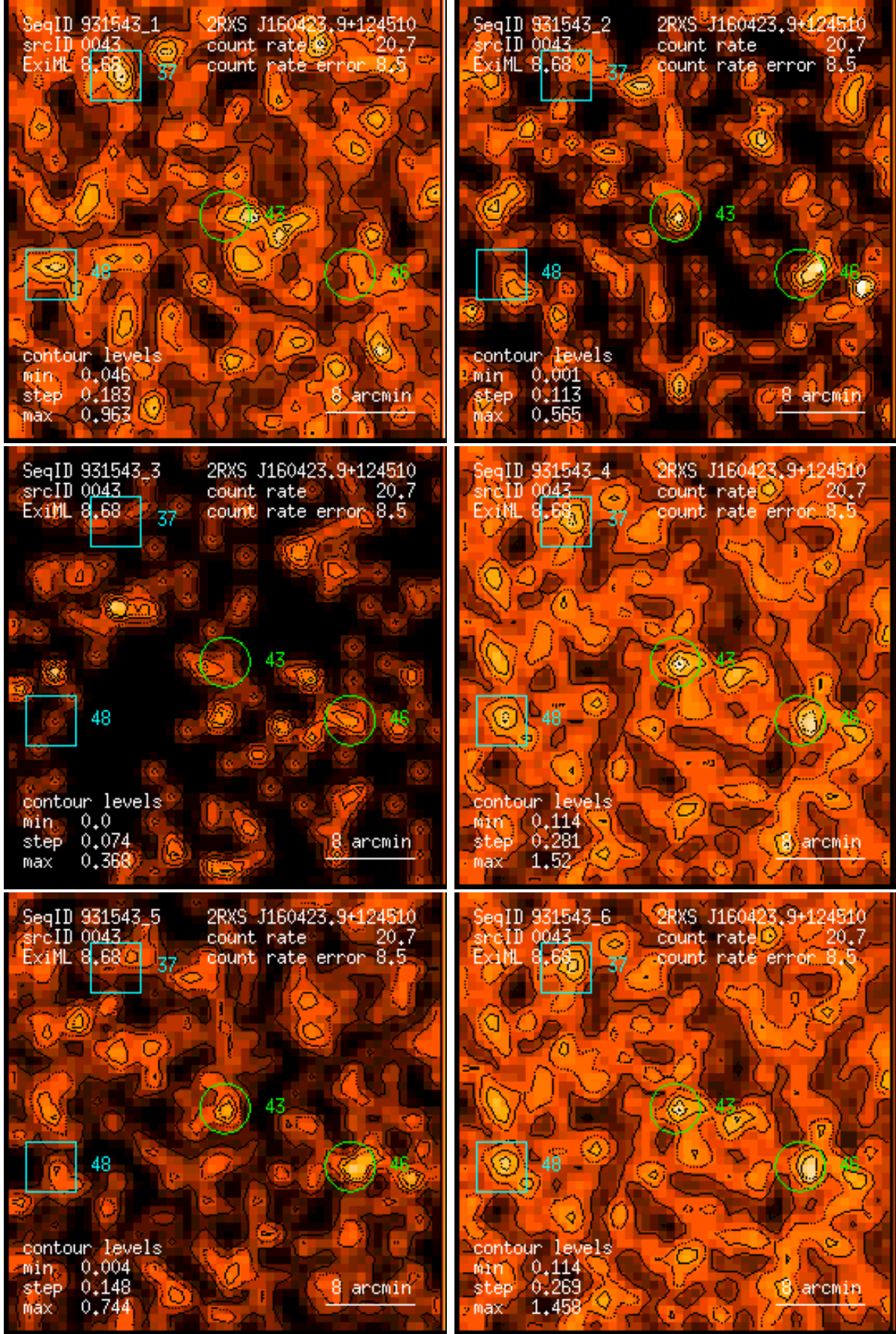
Figure 43: RASS 931543: detection 0043: band rate images, Gaussian filter: (1) PSPC channels 11 – 41, (2) 52 – 90, (3) 91 – 201, (4) 11 – 235, (5) 52 – 201, (6) 11 – 201. Broad band rates in counts/ks. Band rate contour levels in counts/ks/arcmin 2 .
