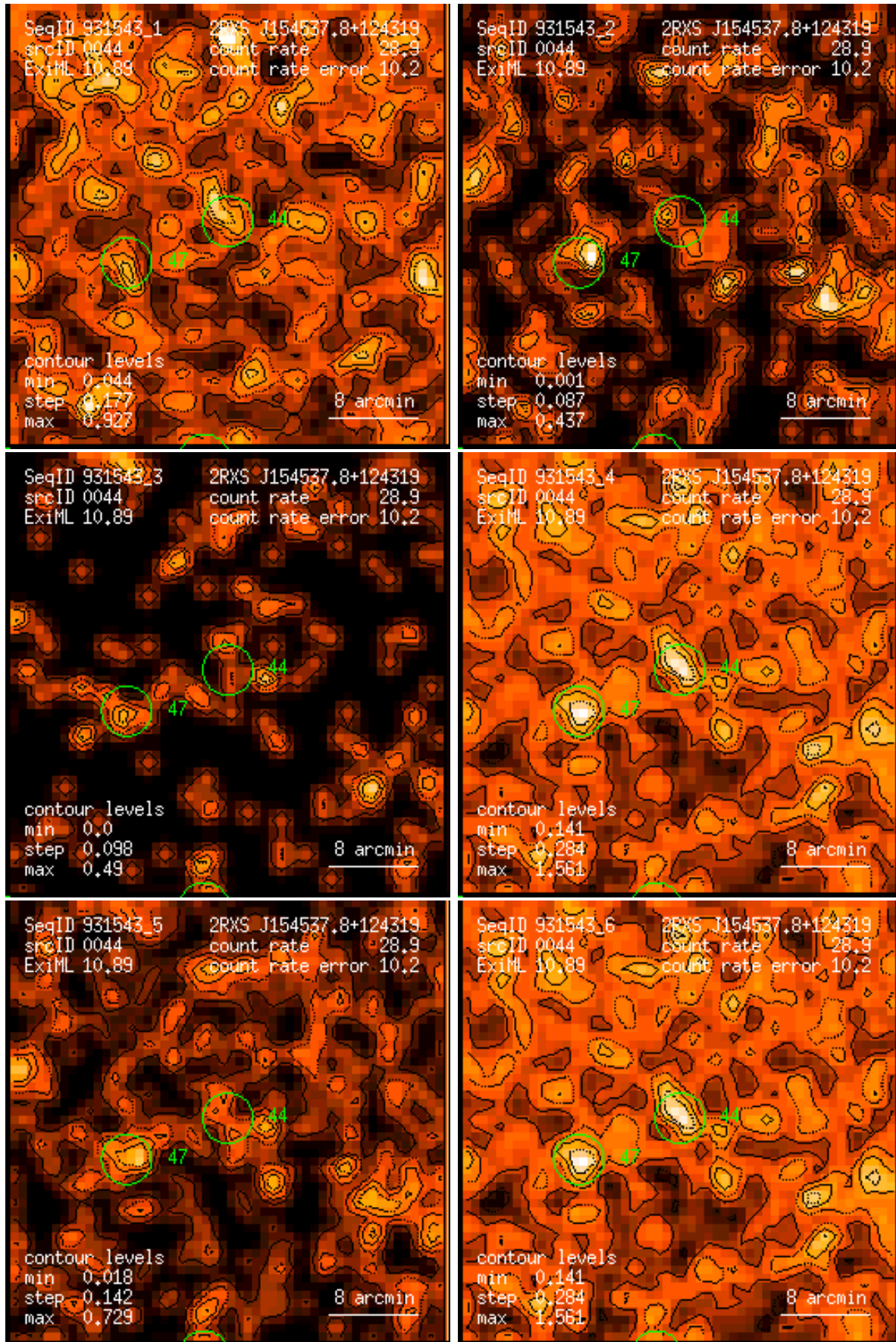
Figure 44: RASS 931543: detection 0044: band rate images, Gaussian filter: (1) PSPC channels 11 – 41, (2) 52 – 90, (3) 91 – 201, (4) 11 – 235, (5) 52 – 201, (6) 11 – 201. Broad band rates in counts/ks. Band rate contour levels in counts/ks/arcmin 2 .
