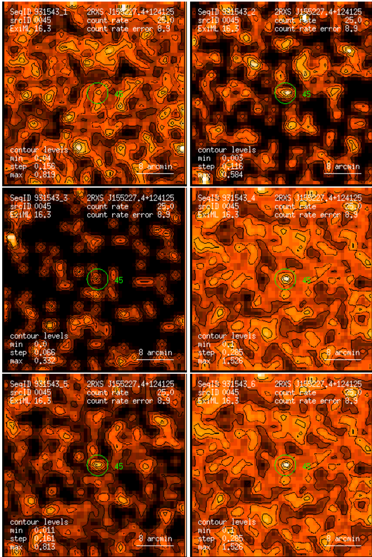
Figure 45: RASS 931543: detection 0045: band rate images, Gaussian filter: (1) PSPC channels 11 – 41, (2) 52 – 90, (3) 91 – 201, (4) 11 – 235, (5) 52 – 201, (6) 11 – 201. Broad band rates in counts/ks. Band rate contour levels in counts/ks/arcmin 2 .
