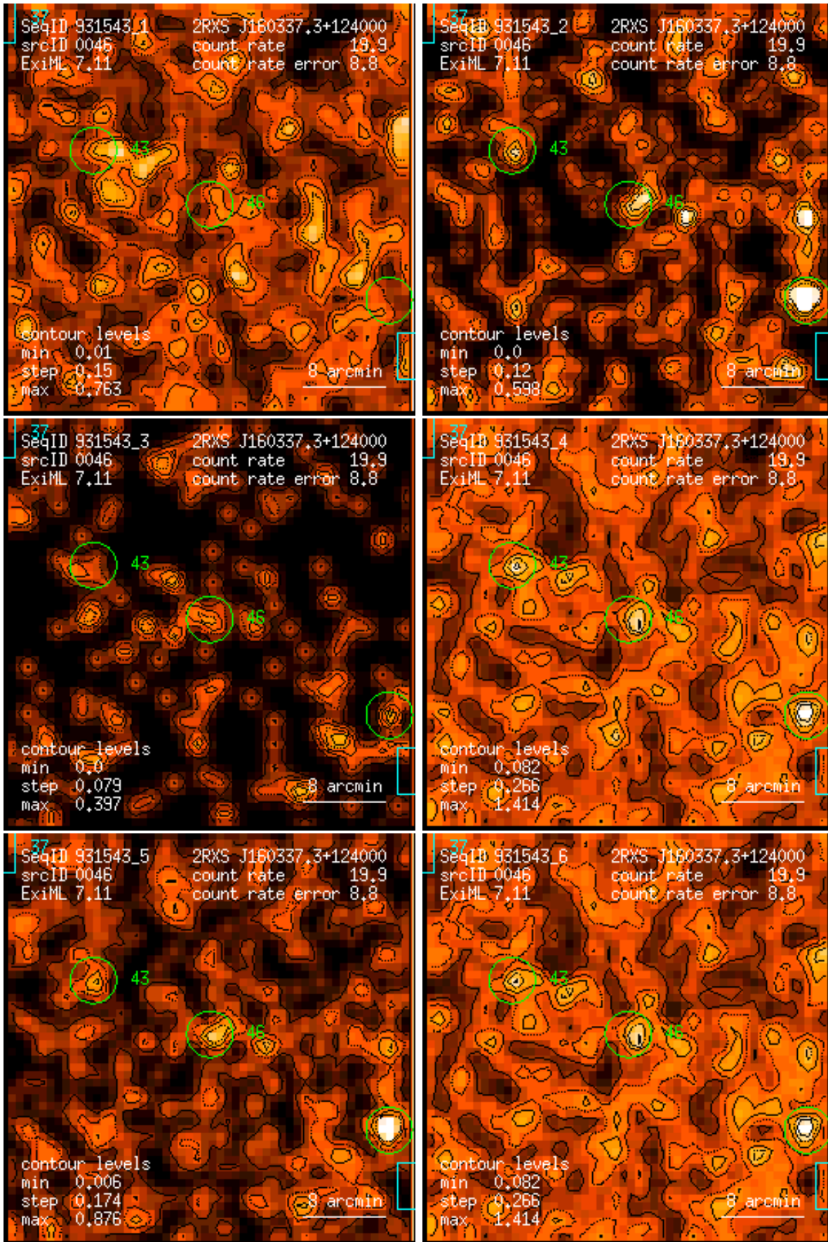
Figure 46: RASS 931543: detection 0046: band rate images, Gaussian filter: (1) PSPC channels 11 – 41, (2) 52 – 90, (3) 91 – 201, (4) 11 – 235, (5) 52 – 201, (6) 11 – 201. Broad band rates in counts/ks. Band rate contour levels in counts/ks/arcmin 2 .
