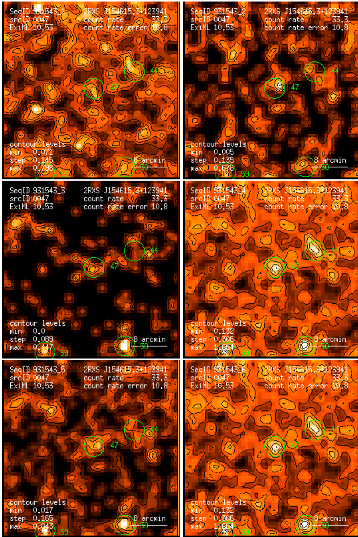
Figure 47: RASS 931543: detection 0047: band rate images, Gaussian filter: (1) PSPC channels 11 – 41, (2) 52 – 90, (3) 91 – 201, (4) 11 – 235, (5) 52 – 201, (6) 11 – 201. Broad band rates in counts/ks. Band rate contour levels in counts/ks/arcmin 2 .
