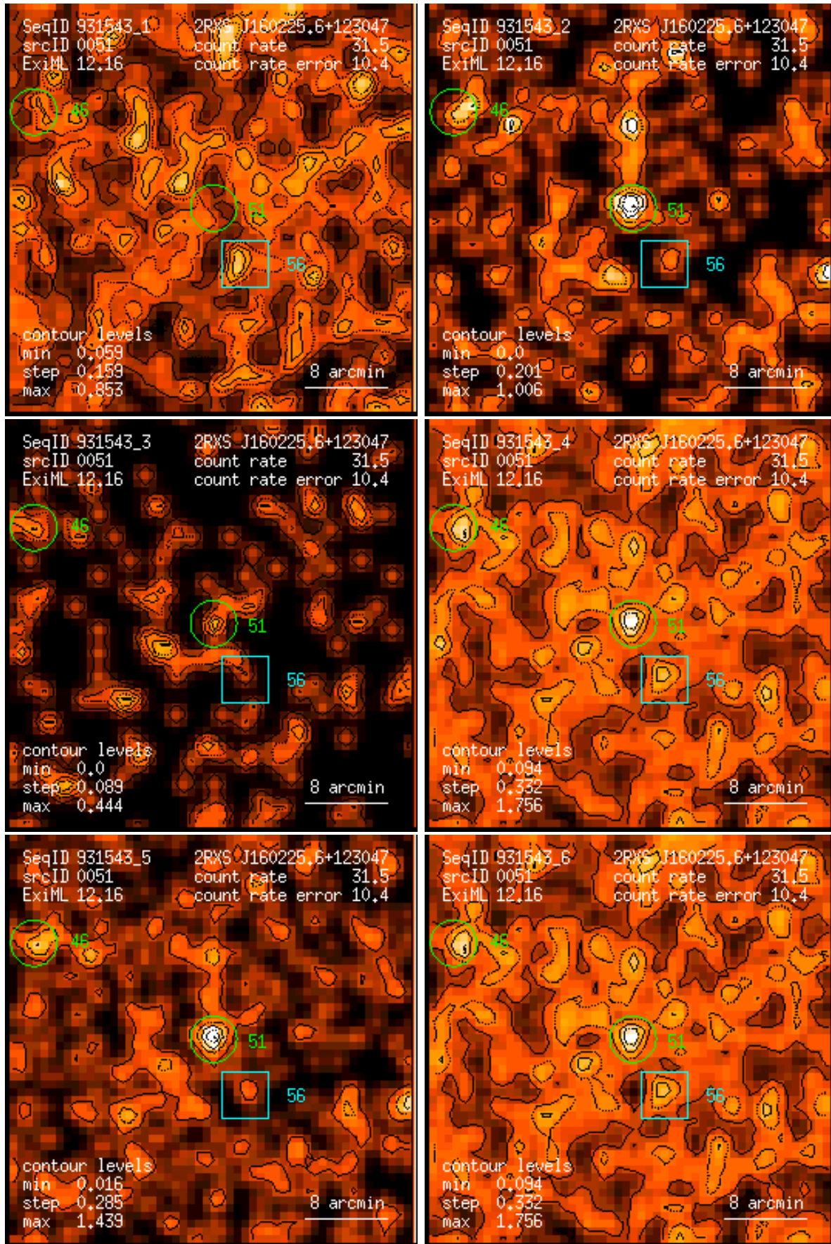
Figure 51: RASS 931543: detection 0051: band rate images, Gaussian filter: (1) PSPC channels 11 – 41, (2) 52 – 90, (3) 91 – 201, (4) 11 – 235, (5) 52 – 201, (6) 11 – 201. Broad band rates in counts/ks. Band rate contour levels in counts/ks/arcmin 2 .
