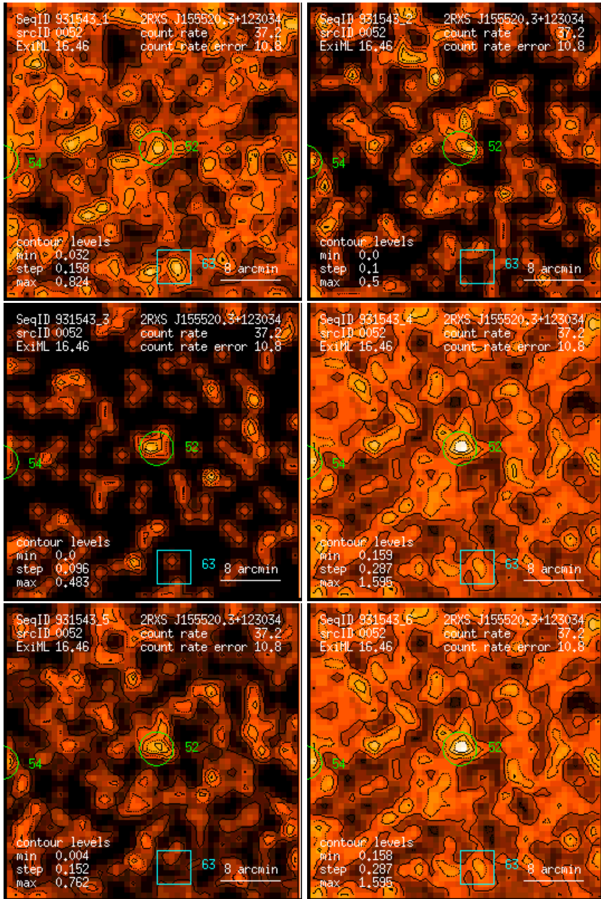
Figure 52: RASS 931543: detection 0052: band rate images, Gaussian filter: (1) PSPC channels 11 – 41, (2) 52 – 90, (3) 91 – 201, (4) 11 – 235, (5) 52 – 201, (6) 11 – 201. Broad band rates in counts/ks. Band rate contour levels in counts/ks/arcmin 2 .
