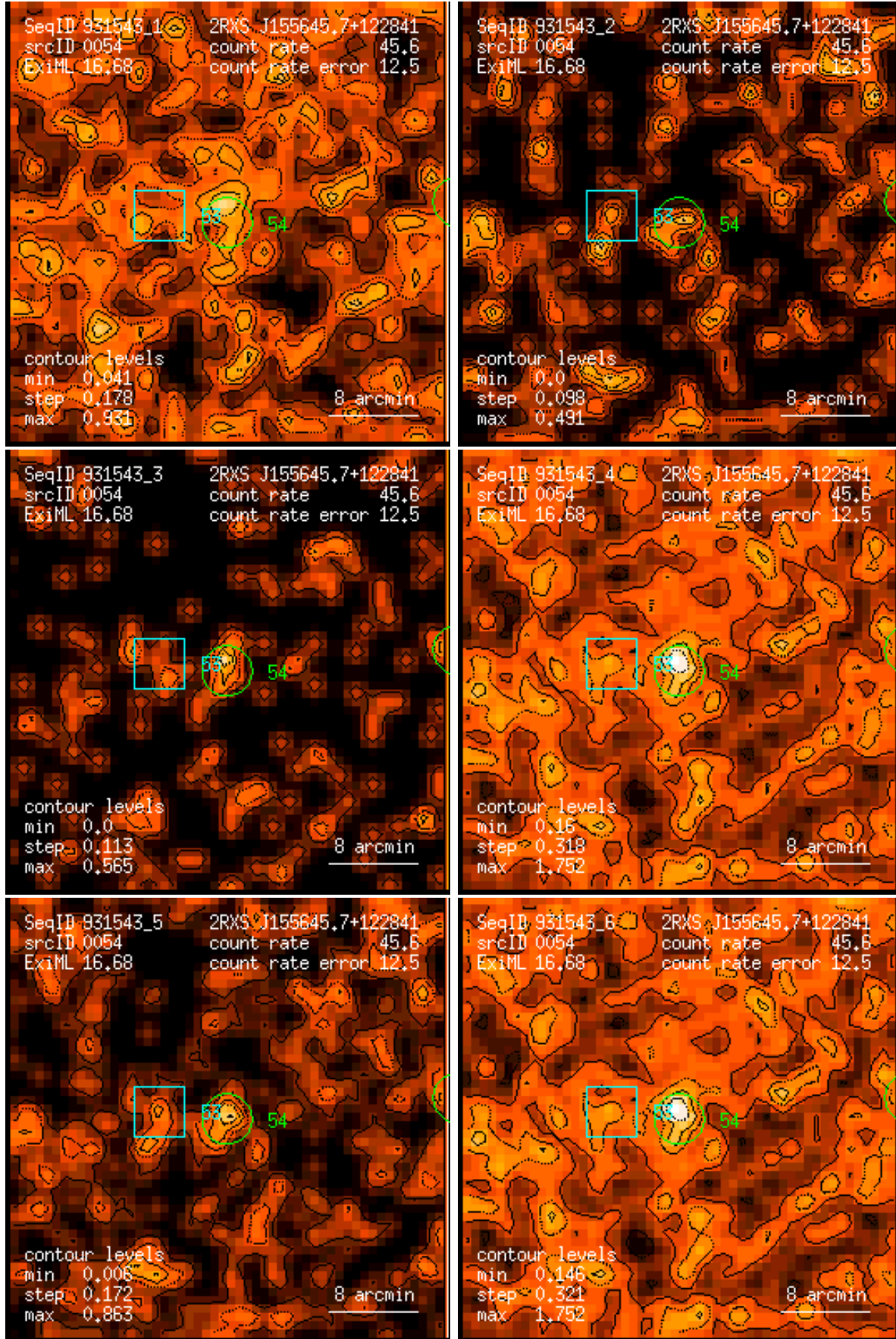
Figure 54: RASS 931543: detection 0054: band rate images, Gaussian filter: (1) PSPC channels 11 – 41, (2) 52 – 90, (3) 91 – 201, (4) 11 – 235, (5) 52 – 201, (6) 11 – 201. Broad band rates in counts/ks. Band rate contour levels in counts/ks/arcmin 2 .
