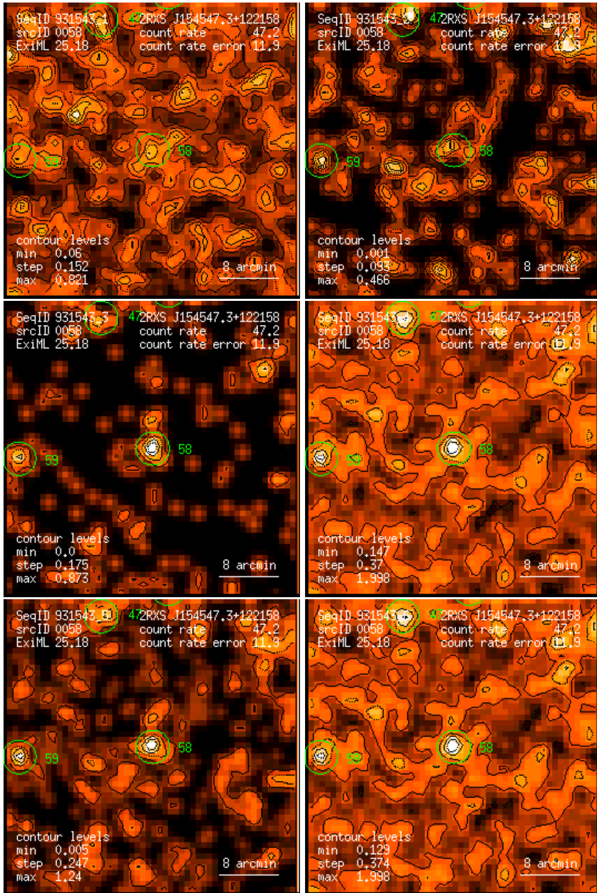
Figure 58: RASS 931543: detection 0058: band rate images, Gaussian filter: (1) PSPC channels 11 – 41, (2) 52 – 90, (3) 91 – 201, (4) 11 – 235, (5) 52 – 201, (6) 11 – 201. Broad band rates in counts/ks. Band rate contour levels in counts/ks/arcmin 2 .
