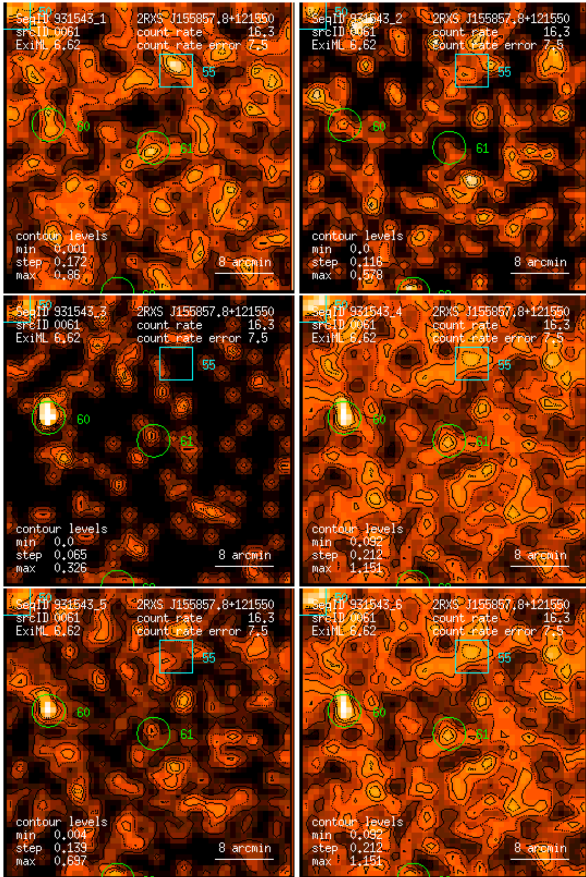
Figure 61: RASS 931543: detection 0061: band rate images, Gaussian filter: (1) PSPC channels 11 – 41, (2) 52 – 90, (3) 91 – 201, (4) 11 – 235, (5) 52 – 201, (6) 11 – 201. Broad band rates in counts/ks. Band rate contour levels in counts/ks/arcmin 2 .
