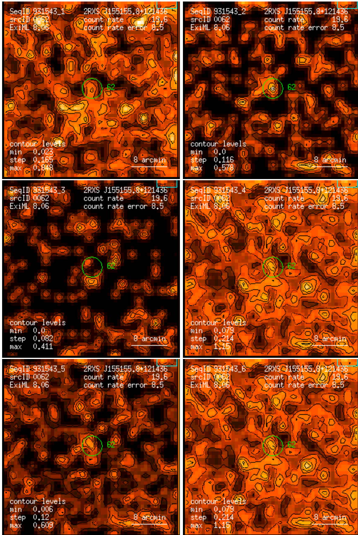
Figure 62: RASS 931543: detection 0062: band rate images, Gaussian filter: (1) PSPC channels 11 – 41, (2) 52 – 90, (3) 91 – 201, (4) 11 – 235, (5) 52 – 201, (6) 11 – 201. Broad band rates in counts/ks. Band rate contour levels in counts/ks/arcmin 2 .
