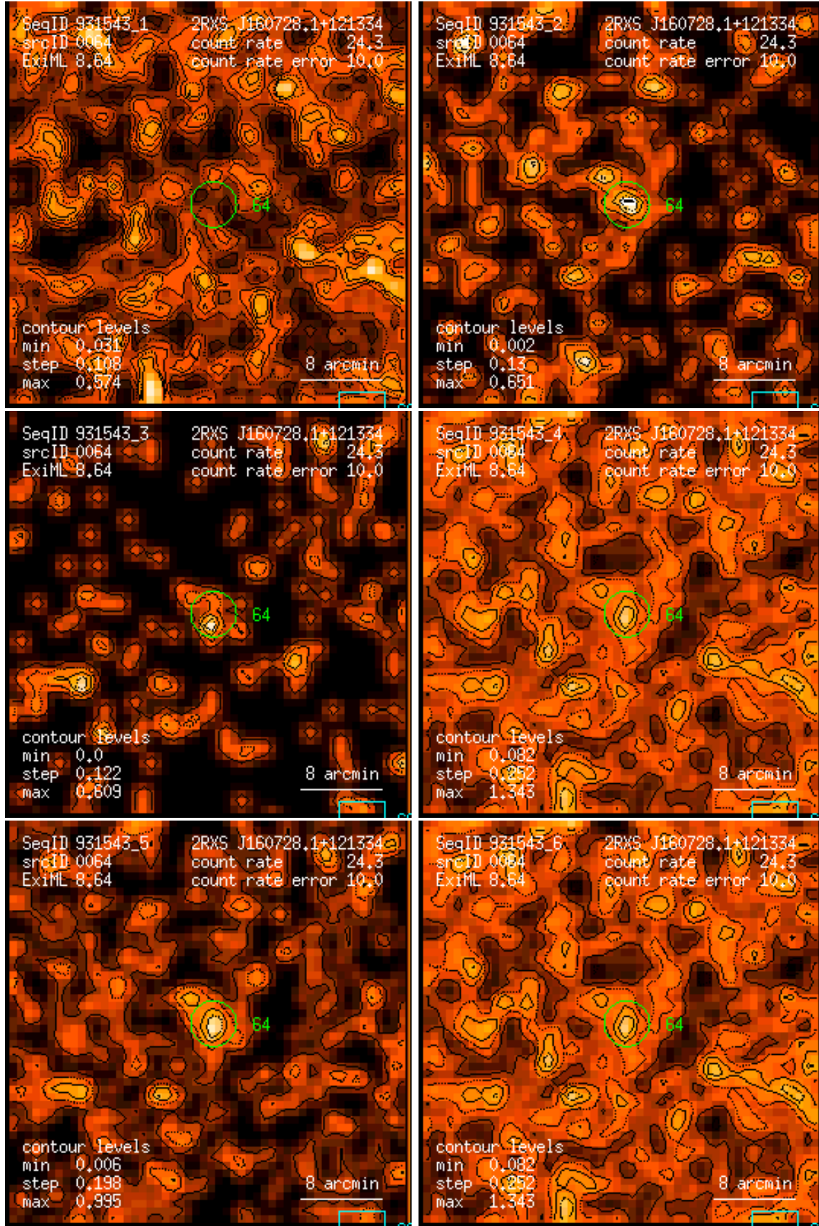
Figure 64: RASS 931543: detection 0064: band rate images, Gaussian filter: (1) PSPC channels 11 – 41, (2) 52 – 90, (3) 91 – 201, (4) 11 – 235, (5) 52 – 201, (6) 11 – 201. Broad band rates in counts/ks. Band rate contour levels in counts/ks/arcmin 2 .
