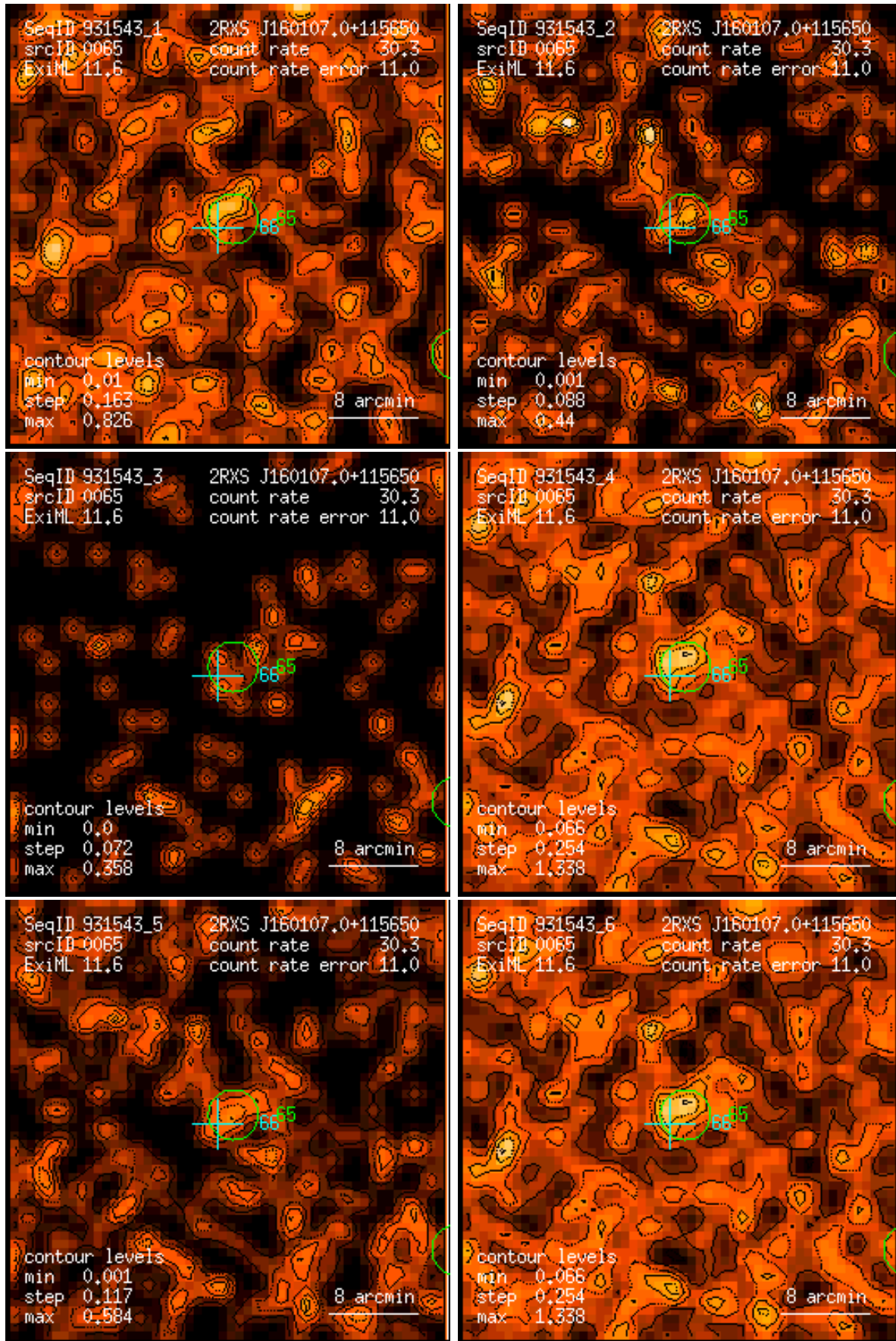
Figure 65: RASS 931543: detection 0065: band rate images, Gaussian filter: (1) PSPC channels 11 – 41, (2) 52 – 90, (3) 91 – 201, (4) 11 – 235, (5) 52 – 201, (6) 11 – 201. Broad band rates in counts/ks. Band rate contour levels in counts/ks/arcmin 2 .
