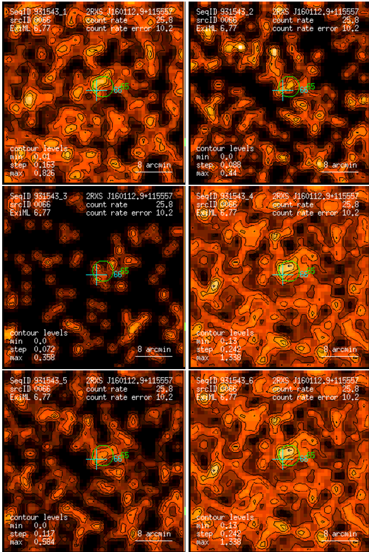
Figure 66: RASS 931543: detection 0066: band rate images, Gaussian filter: (1) PSPC channels 11 – 41, (2) 52 – 90, (3) 91 – 201, (4) 11 – 235, (5) 52 – 201, (6) 11 – 201. Broad band rates in counts/ks. Band rate contour levels in counts/ks/arcmin 2 .
