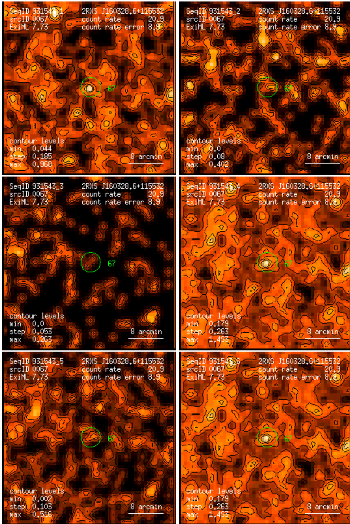
Figure 67: RASS 931543: detection 0067: band rate images, Gaussian filter: (1) PSPC channels 11 – 41, (2) 52 – 90, (3) 91 – 201, (4) 11 – 235, (5) 52 – 201, (6) 11 – 201. Broad band rates in counts/ks. Band rate contour levels in counts/ks/arcmin 2 .
