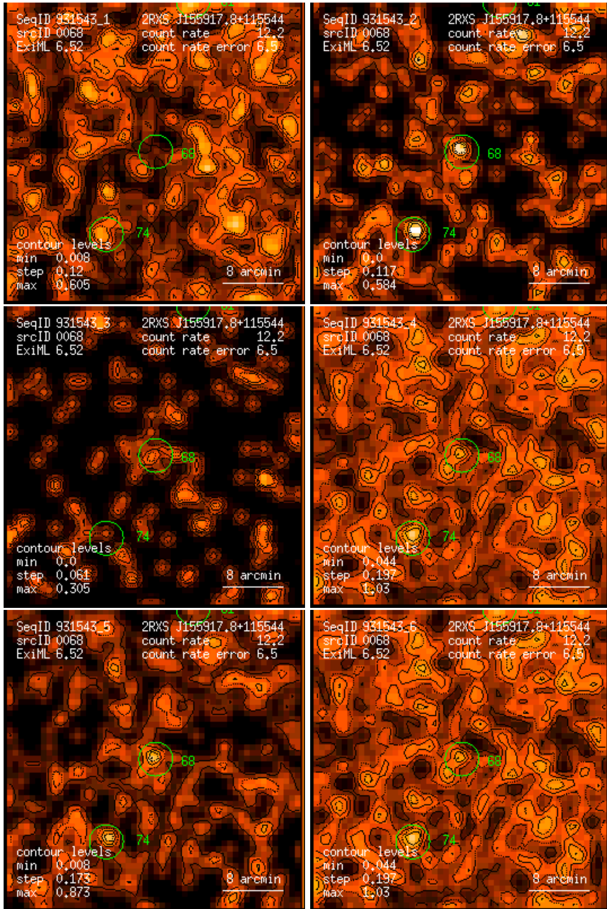
Figure 68: RASS 931543: detection 0068: band rate images, Gaussian filter: (1) PSPC channels 11 – 41, (2) 52 – 90, (3) 91 – 201, (4) 11 – 235, (5) 52 – 201, (6) 11 – 201. Broad band rates in counts/ks. Band rate contour levels in counts/ks/arcmin 2 .
