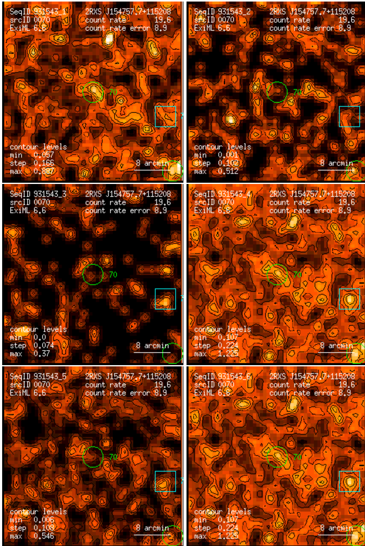
Figure 70: RASS 931543: detection 0070: band rate images, Gaussian filter: (1) PSPC channels 11 – 41, (2) 52 – 90, (3) 91 – 201, (4) 11 – 235, (5) 52 – 201, (6) 11 – 201. Broad band rates in counts/ks. Band rate contour levels in counts/ks/arcmin 2 .
