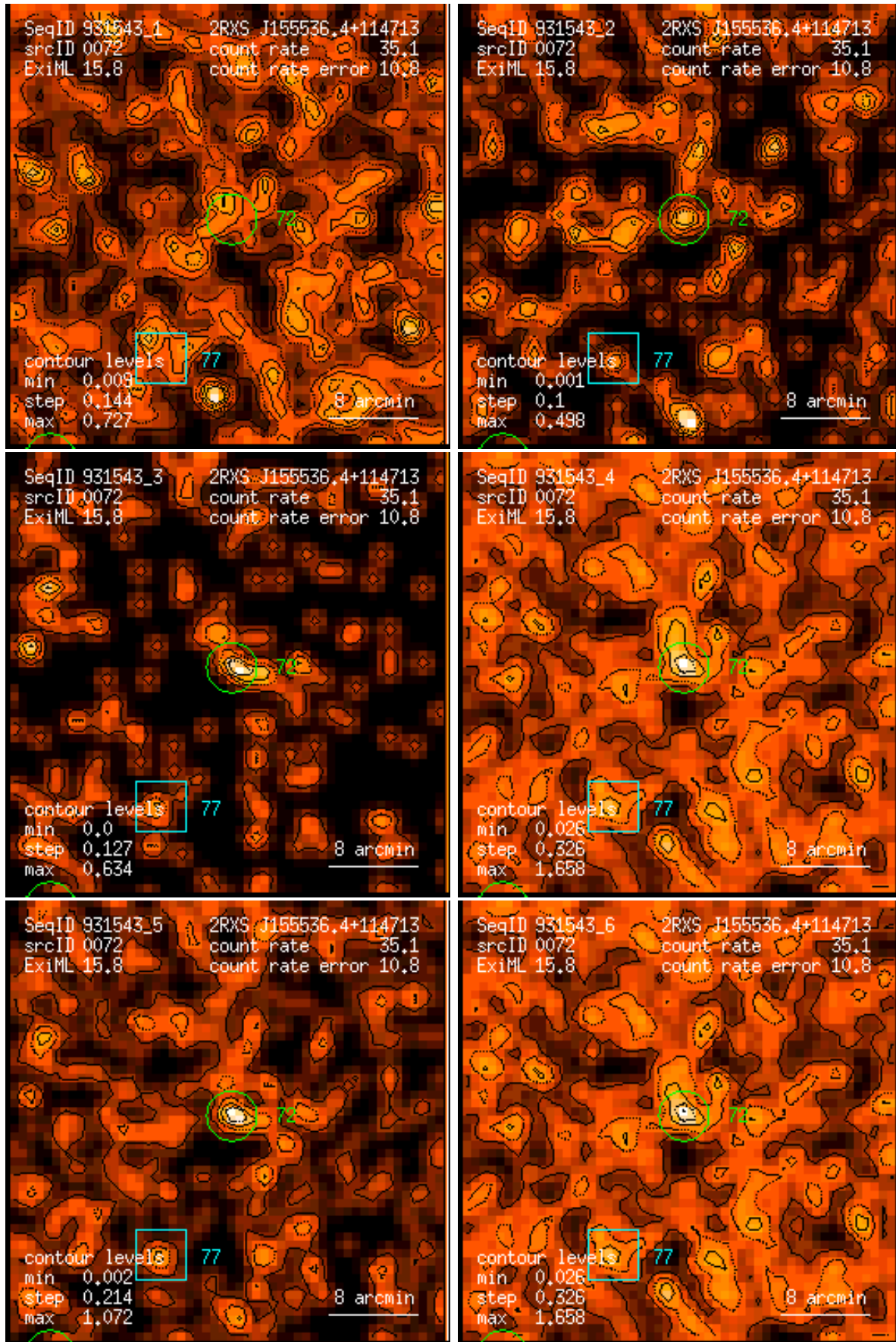
Figure 72: RASS 931543: detection 0072: band rate images, Gaussian filter: (1) PSPC channels 11 – 41, (2) 52 – 90, (3) 91 – 201, (4) 11 – 235, (5) 52 – 201, (6) 11 – 201. Broad band rates in counts/ks. Band rate contour levels in counts/ks/arcmin 2 .
