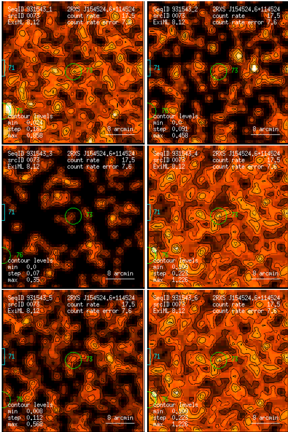
Figure 73: RASS 931543: detection 0073: band rate images, Gaussian filter: (1) PSPC channels 11 – 41, (2) 52 – 90, (3) 91 – 201, (4) 11 – 235, (5) 52 – 201, (6) 11 – 201. Broad band rates in counts/ks. Band rate contour levels in counts/ks/arcmin 2 .
