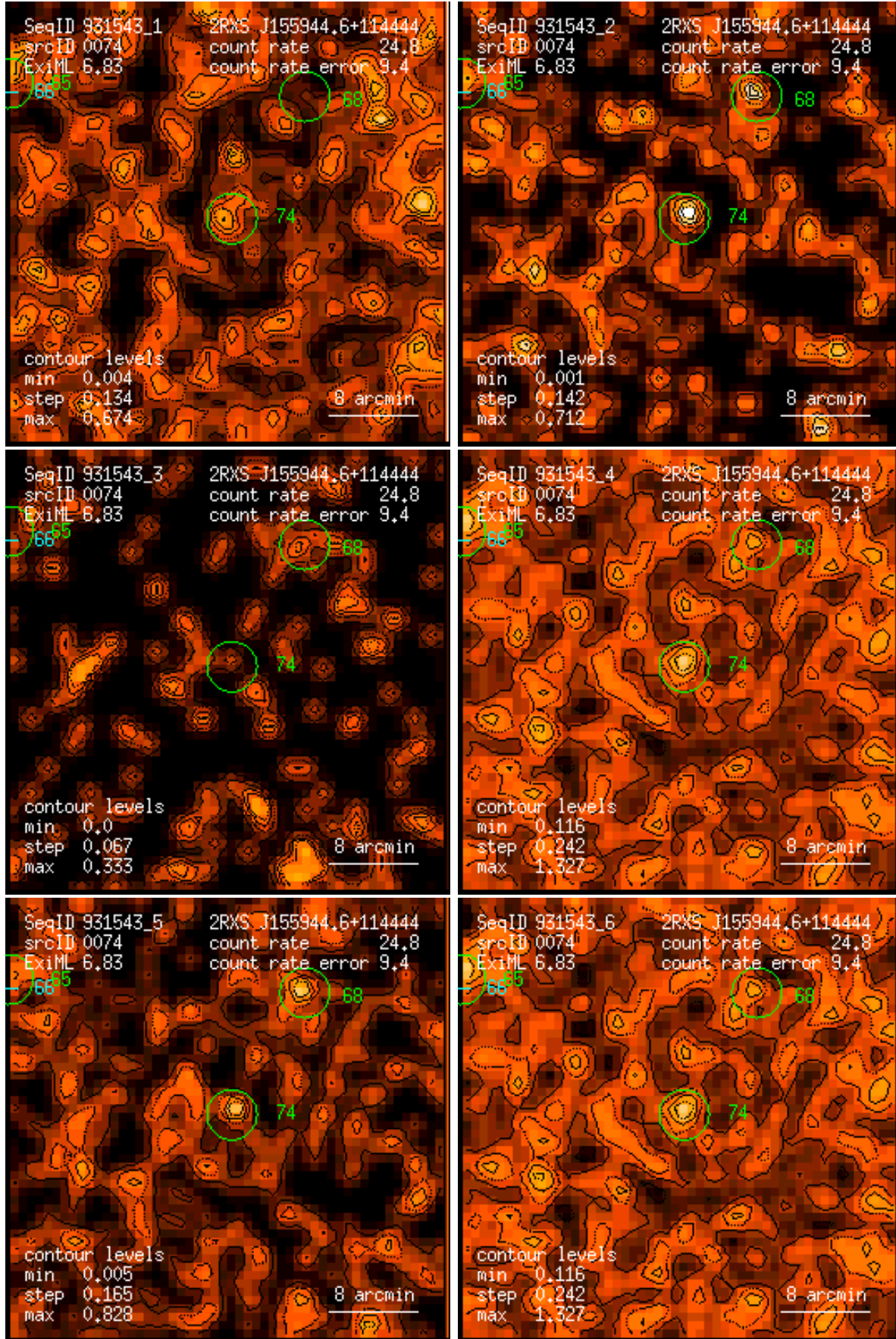
Figure 74: RASS 931543: detection 0074: band rate images, Gaussian filter: (1) PSPC channels 11 – 41, (2) 52 – 90, (3) 91 – 201, (4) 11 – 235, (5) 52 – 201, (6) 11 – 201. Broad band rates in counts/ks. Band rate contour levels in counts/ks/arcmin 2 .
