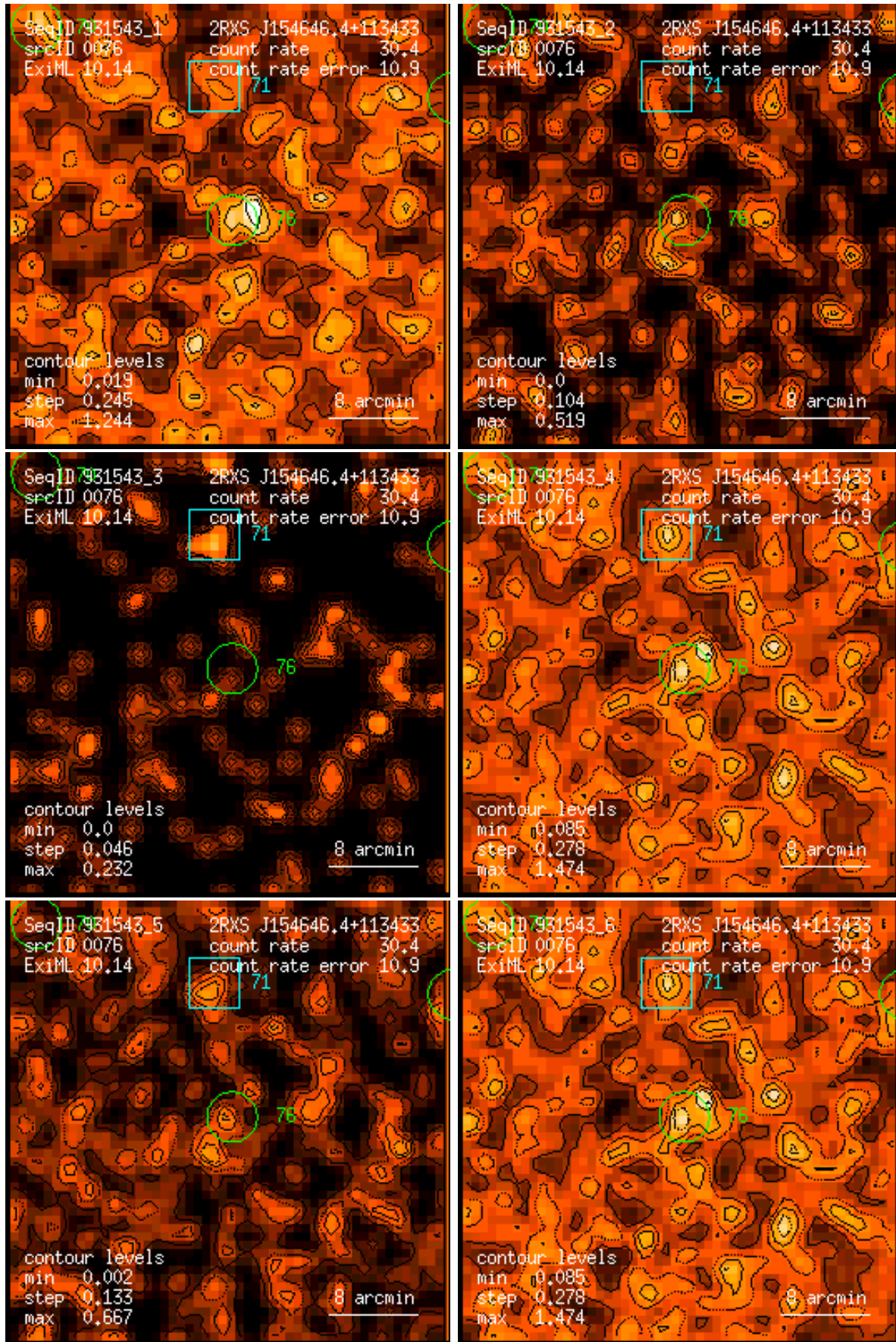
Figure 76: RASS 931543: detection 0076: band rate images, Gaussian filter: (1) PSPC channels 11 – 41, (2) 52 – 90, (3) 91 – 201, (4) 11 – 235, (5) 52 – 201, (6) 11 – 201. Broad band rates in counts/ks. Band rate contour levels in counts/ks/arcmin 2 .
