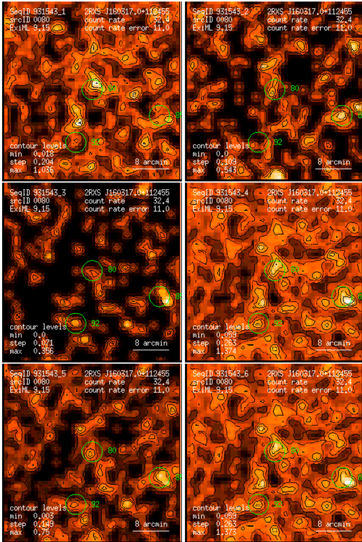
Figure 80: RASS 931543: detection 0080: band rate images, Gaussian filter: (1) PSPC channels 11 – 41, (2) 52 – 90, (3) 91 – 201, (4) 11 – 235, (5) 52 – 201, (6) 11 – 201. Broad band rates in counts/ks. Band rate contour levels in counts/ks/arcmin 2 .
