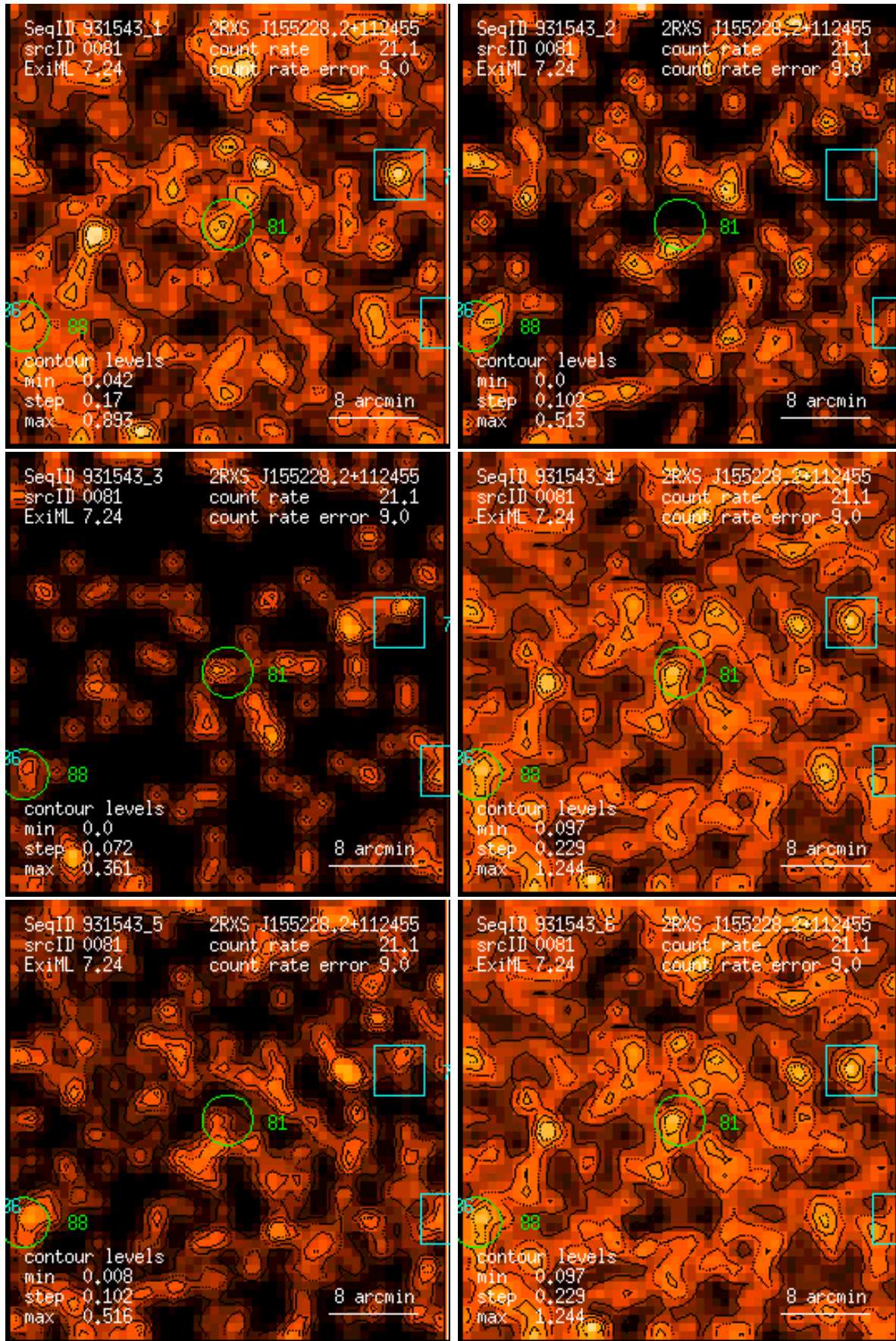
Figure 81: RASS 931543: detection 0081: band rate images, Gaussian filter: (1) PSPC channels 11 – 41, (2) 52 – 90, (3) 91 – 201, (4) 11 – 235, (5) 52 – 201, (6) 11 – 201. Broad band rates in counts/ks. Band rate contour levels in counts/ks/arcmin 2 .
