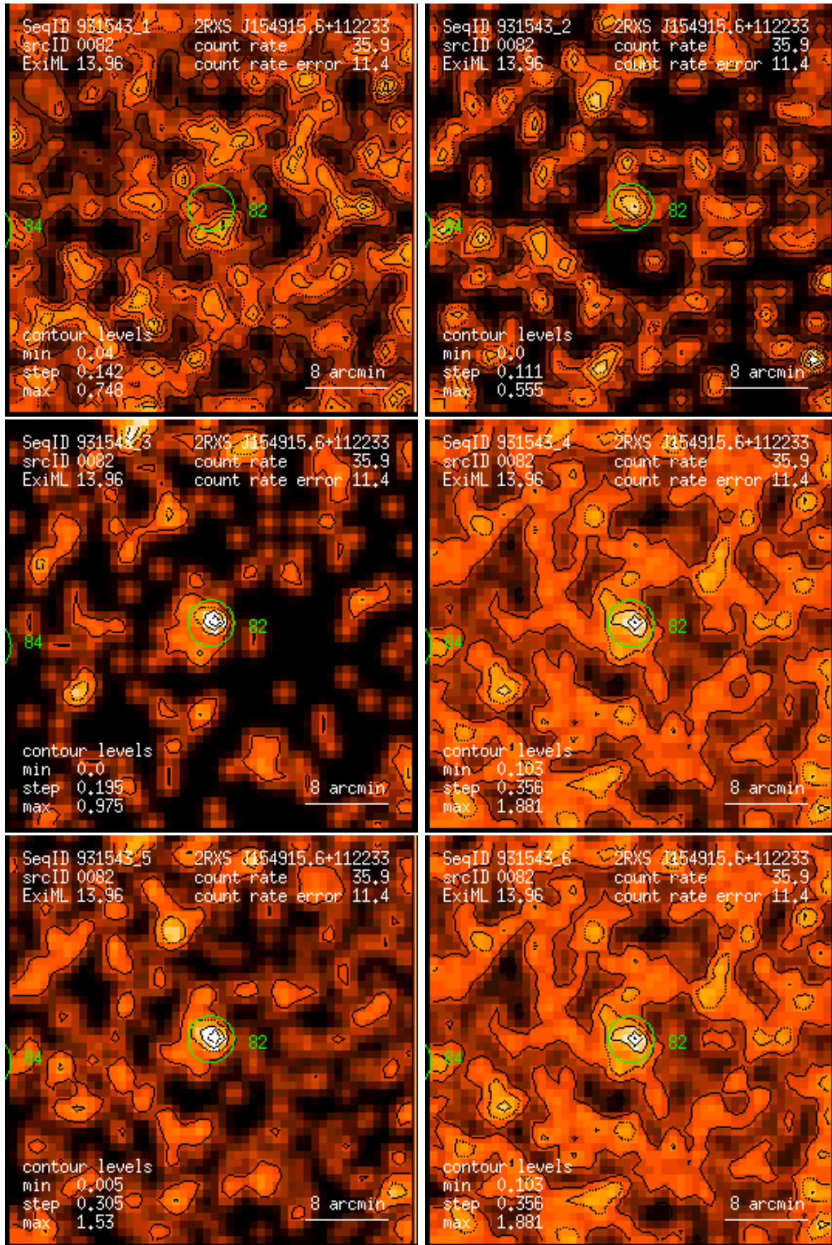
Figure 82: RASS 931543: detection 0082: band rate images, Gaussian filter: (1) PSPC channels 11 – 41, (2) 52 – 90, (3) 91 – 201, (4) 11 – 235, (5) 52 – 201, (6) 11 – 201. Broad band rates in counts/ks. Band rate contour levels in counts/ks/arcmin 2 .
