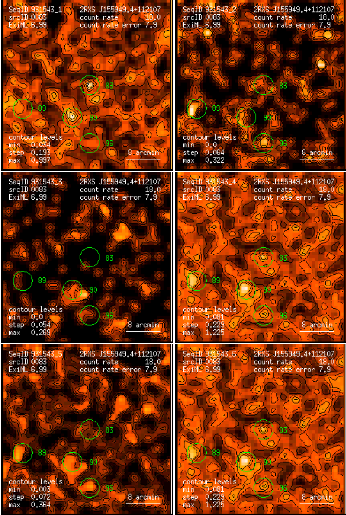
Figure 83: RASS 931543: detection 0083: band rate images, Gaussian filter: (1) PSPC channels 11 – 41, (2) 52 – 90, (3) 91 – 201, (4) 11 – 235, (5) 52 – 201, (6) 11 – 201. Broad band rates in counts/ks. Band rate contour levels in counts/ks/arcmin 2 .
