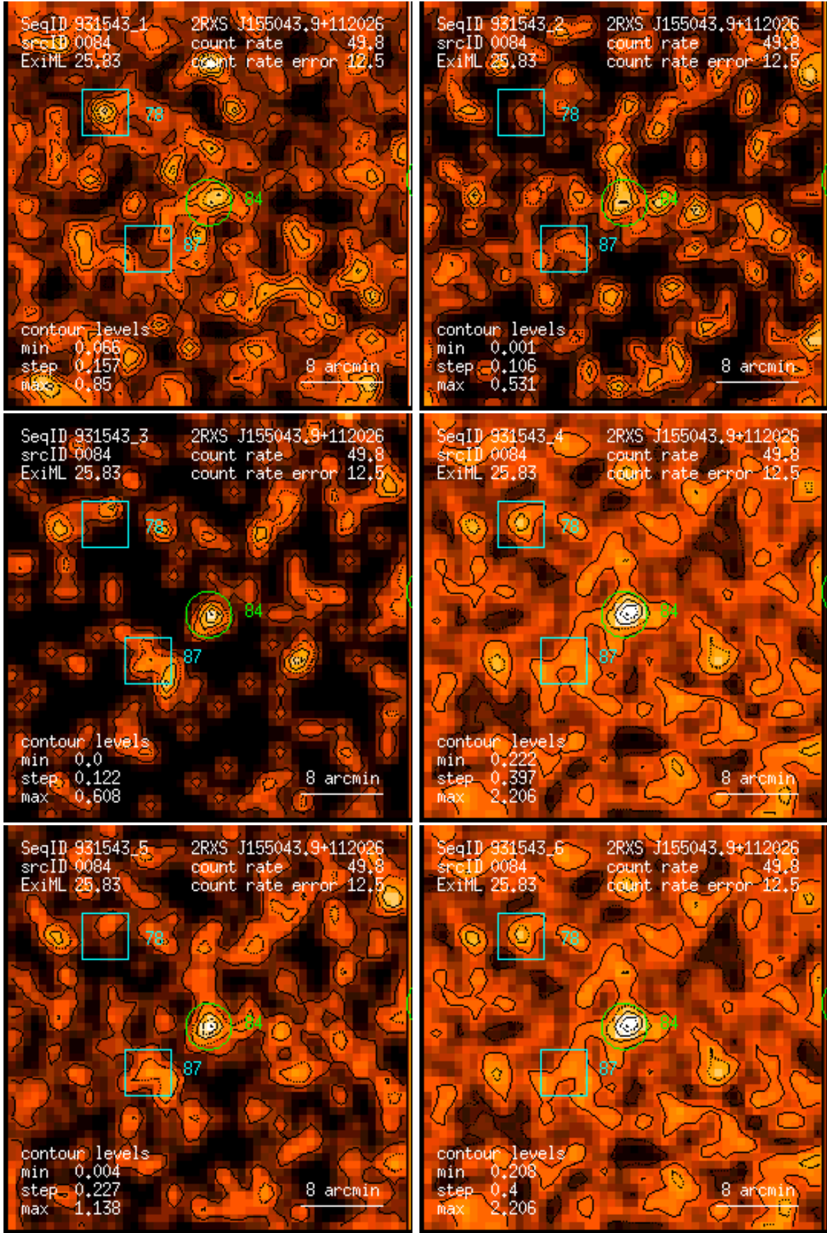
Figure 84: RASS 931543: detection 0084: band rate images, Gaussian filter: (1) PSPC channels 11 – 41, (2) 52 – 90, (3) 91 – 201, (4) 11 – 235, (5) 52 – 201, (6) 11 – 201. Broad band rates in counts/ks. Band rate contour levels in counts/ks/arcmin 2 .
