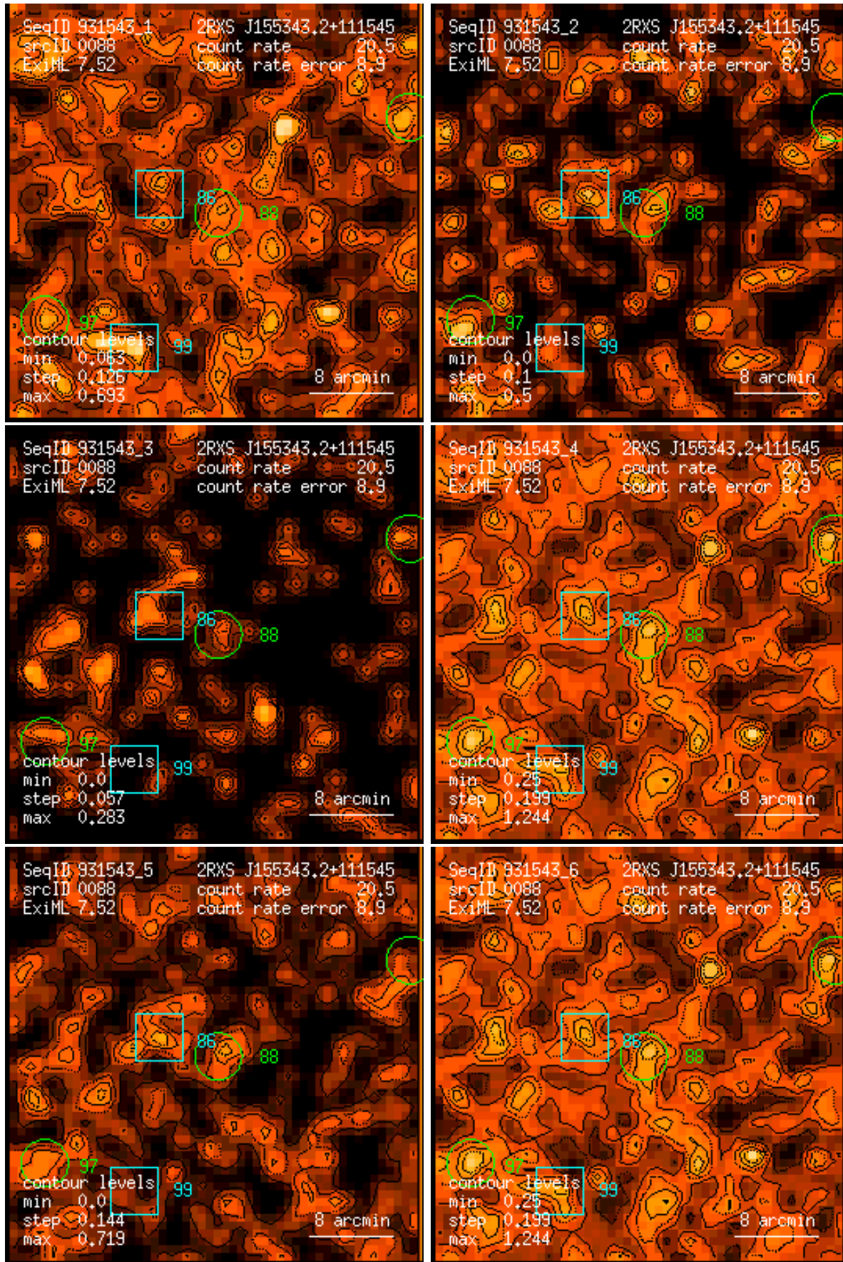
Figure 88: RASS 931543: detection 0088: band rate images, Gaussian filter: (1) PSPC channels 11 – 41, (2) 52 – 90, (3) 91 – 201, (4) 11 – 235, (5) 52 – 201, (6) 11 – 201. Broad band rates in counts/ks. Band rate contour levels in counts/ks/arcmin 2 .
