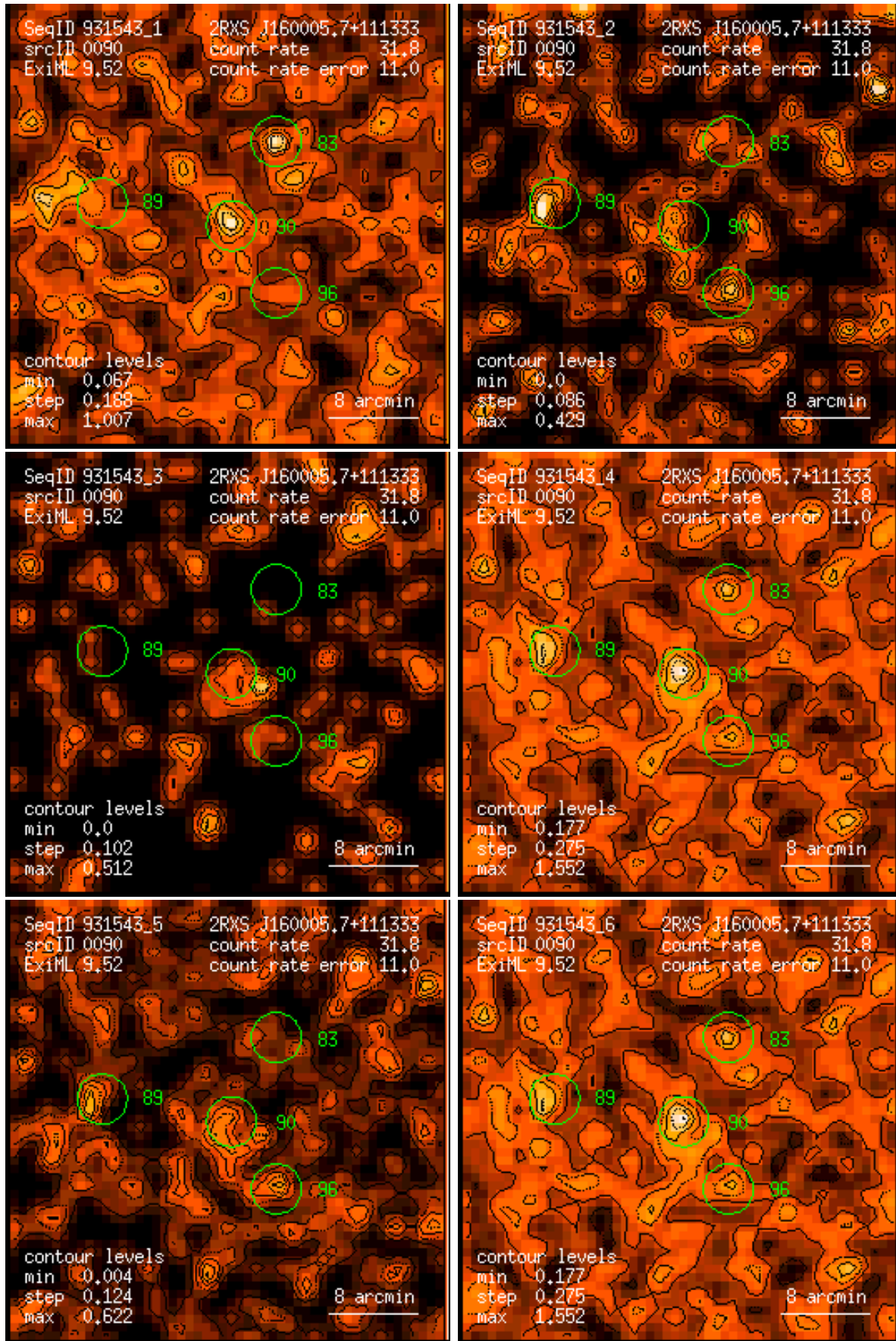
Figure 90: RASS 931543: detection 0090: band rate images, Gaussian filter: (1) PSPC channels 11 – 41, (2) 52 – 90, (3) 91 – 201, (4) 11 – 235, (5) 52 – 201, (6) 11 – 201. Broad band rates in counts/ks. Band rate contour levels in counts/ks/arcmin 2 .
