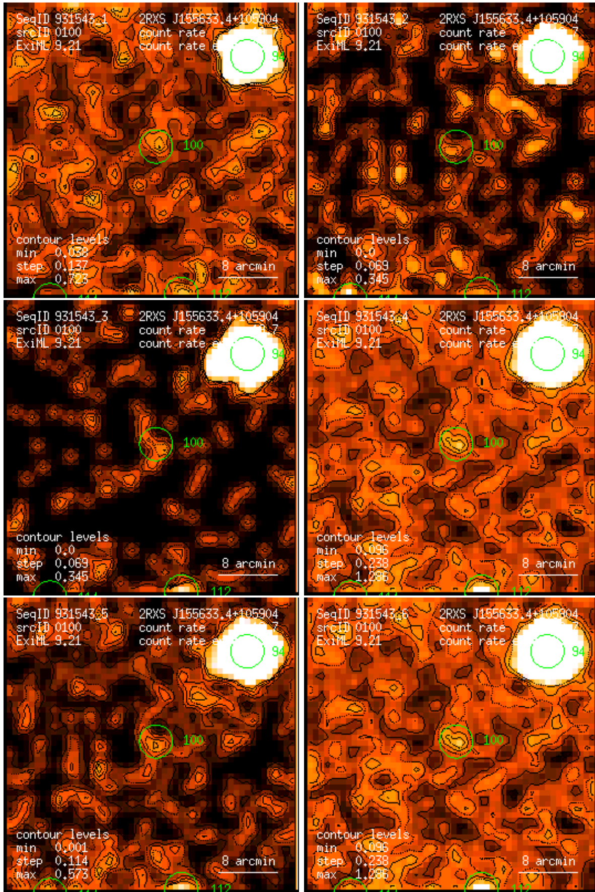
Figure 100: RASS 931543: detection 0100: band rate images, Gaussian filter: (1) PSPC channels 11 – 41, (2) 52 – 90, (3) 91 – 201, (4) 11 – 235, (5) 52 – 201, (6) 11 – 201. Broad band rates in counts/ks. Band rate contour levels in counts/ks/arcmin 2 .
