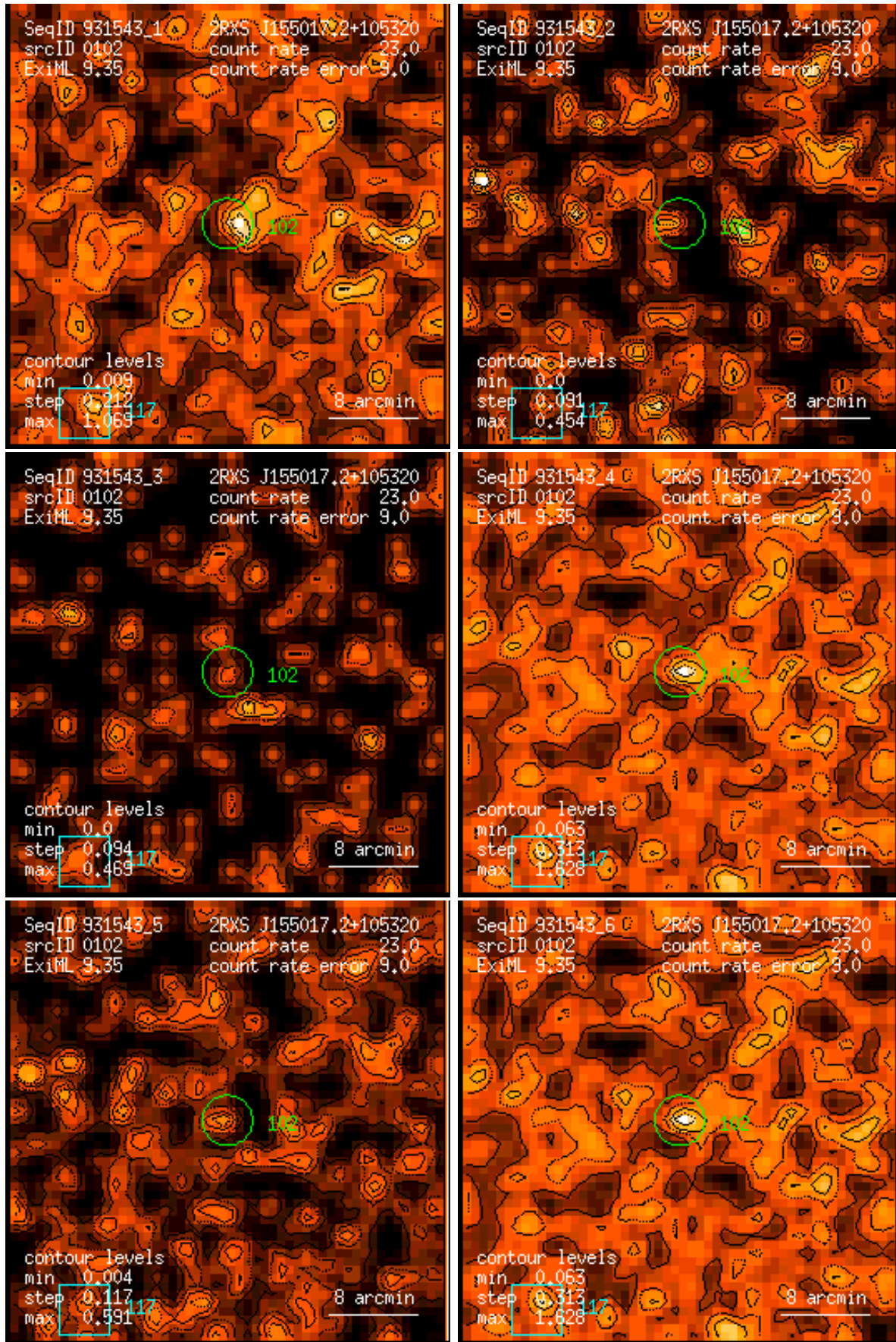
Figure 102: RASS 931543: detection 0102: band rate images, Gaussian filter: (1) PSPC channels 11 – 41, (2) 52 – 90, (3) 91 – 201, (4) 11 – 235, (5) 52 – 201, (6) 11 – 201. Broad band rates in counts/ks. Band rate contour levels in counts/ks/arcmin 2 .
