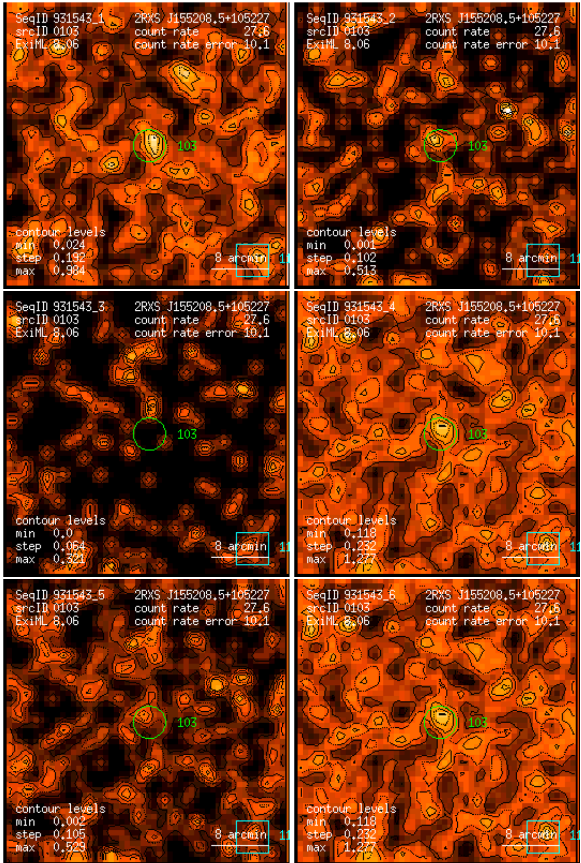
Figure 103: RASS 931543: detection 0103: band rate images, Gaussian filter: (1) PSPC channels 11 – 41, (2) 52 – 90, (3) 91 – 201, (4) 11 – 235, (5) 52 – 201, (6) 11 – 201. Broad band rates in counts/ks. Band rate contour levels in counts/ks/arcmin 2 .
