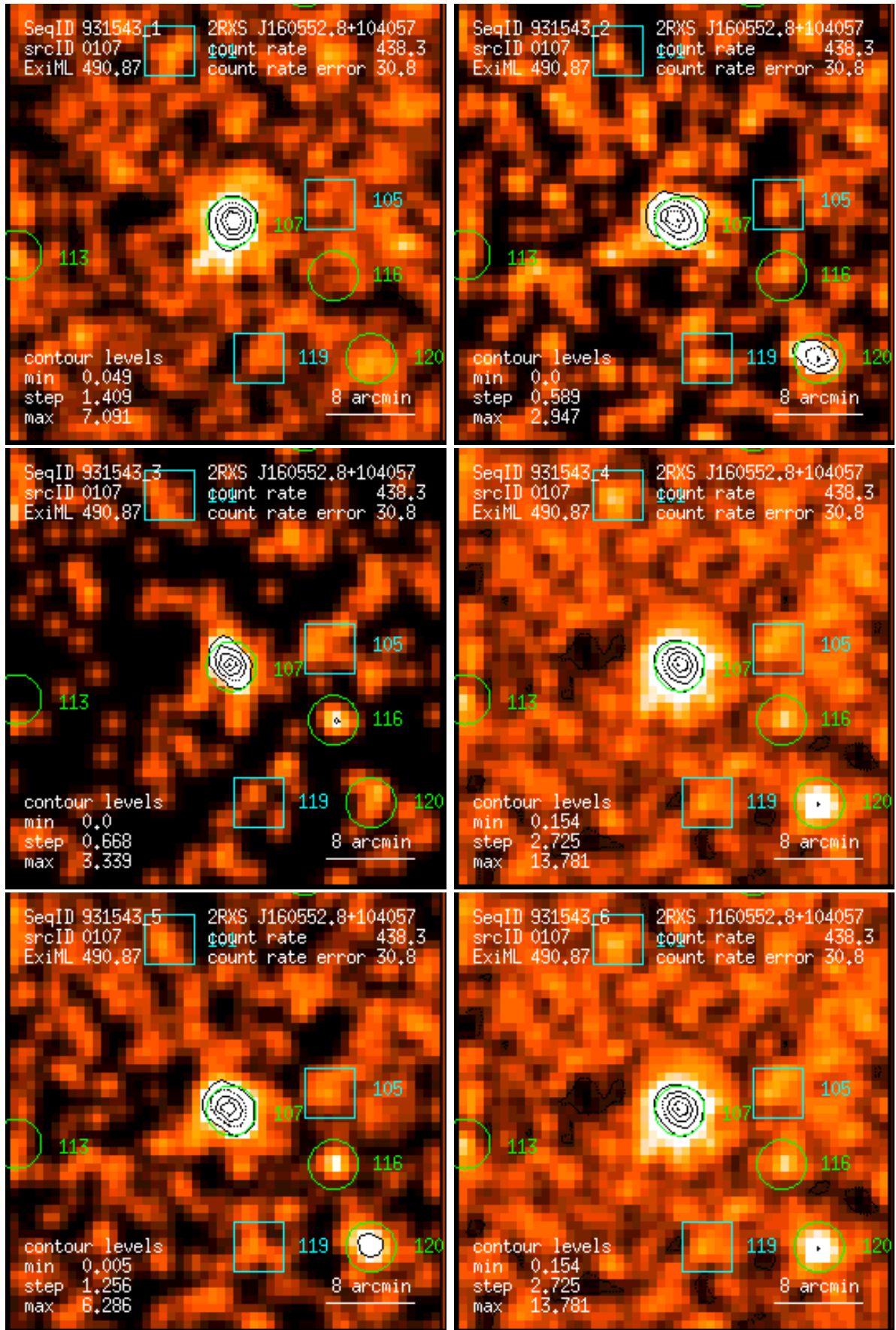
Figure 107: RASS 931543: detection 0107: band rate images, Gaussian filter: (1) PSPC channels 11 – 41, (2) 52 – 90, (3) 91 – 201, (4) 11 – 235, (5) 52 – 201, (6) 11 – 201. Broad band rates in counts/ks. Band rate contour levels in counts/ks/arcmin 2 .
