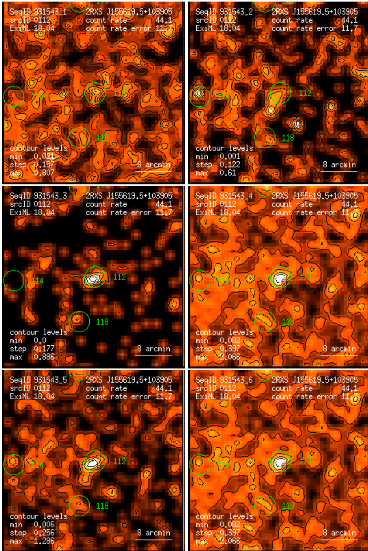
Figure 112: RASS 931543: detection 0112: band rate images, Gaussian filter: (1) PSPC channels 11 – 41, (2) 52 – 90, (3) 91 – 201, (4) 11 – 235, (5) 52 – 201, (6) 11 – 201. Broad band rates in counts/ks. Band rate contour levels in counts/ks/arcmin 2 .
