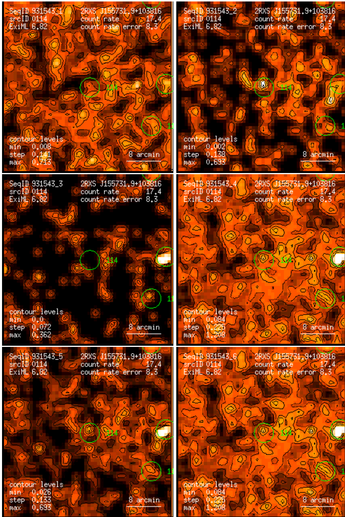
Figure 114: RASS 931543: detection 0114: band rate images, Gaussian filter: (1) PSPC channels 11 – 41, (2) 52 – 90, (3) 91 – 201, (4) 11 – 235, (5) 52 – 201, (6) 11 – 201. Broad band rates in counts/ks. Band rate contour levels in counts/ks/arcmin 2 .
