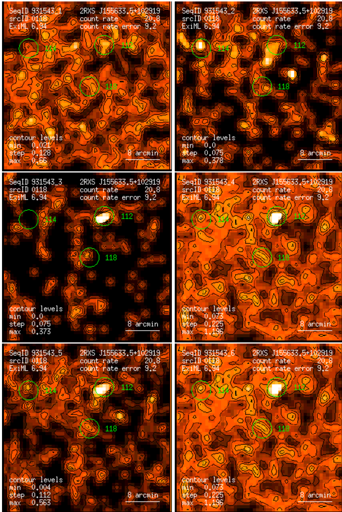
Figure 118: RASS 931543: detection 0118: band rate images, Gaussian filter: (1) PSPC channels 11 – 41, (2) 52 – 90, (3) 91 – 201, (4) 11 – 235, (5) 52 – 201, (6) 11 – 201. Broad band rates in counts/ks. Band rate contour levels in counts/ks/arcmin 2 .
