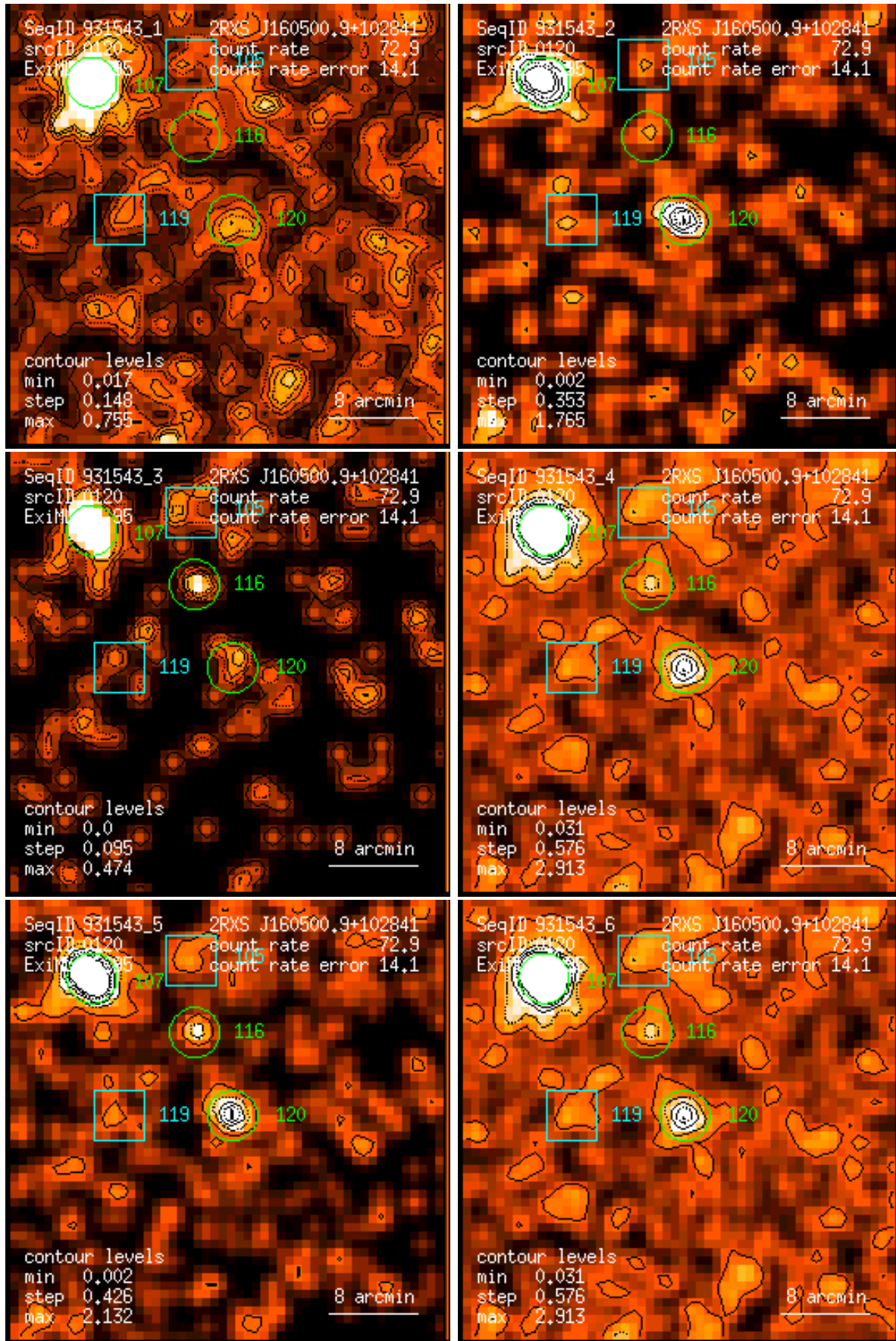
Figure 120: RASS 931543: detection 0120: band rate images, Gaussian filter: (1) PSPC channels 11 – 41, (2) 52 – 90, (3) 91 – 201, (4) 11 – 235, (5) 52 – 201, (6) 11 – 201. Broad band rates in counts/ks. Band rate contour levels in counts/ks/arcmin 2 .
