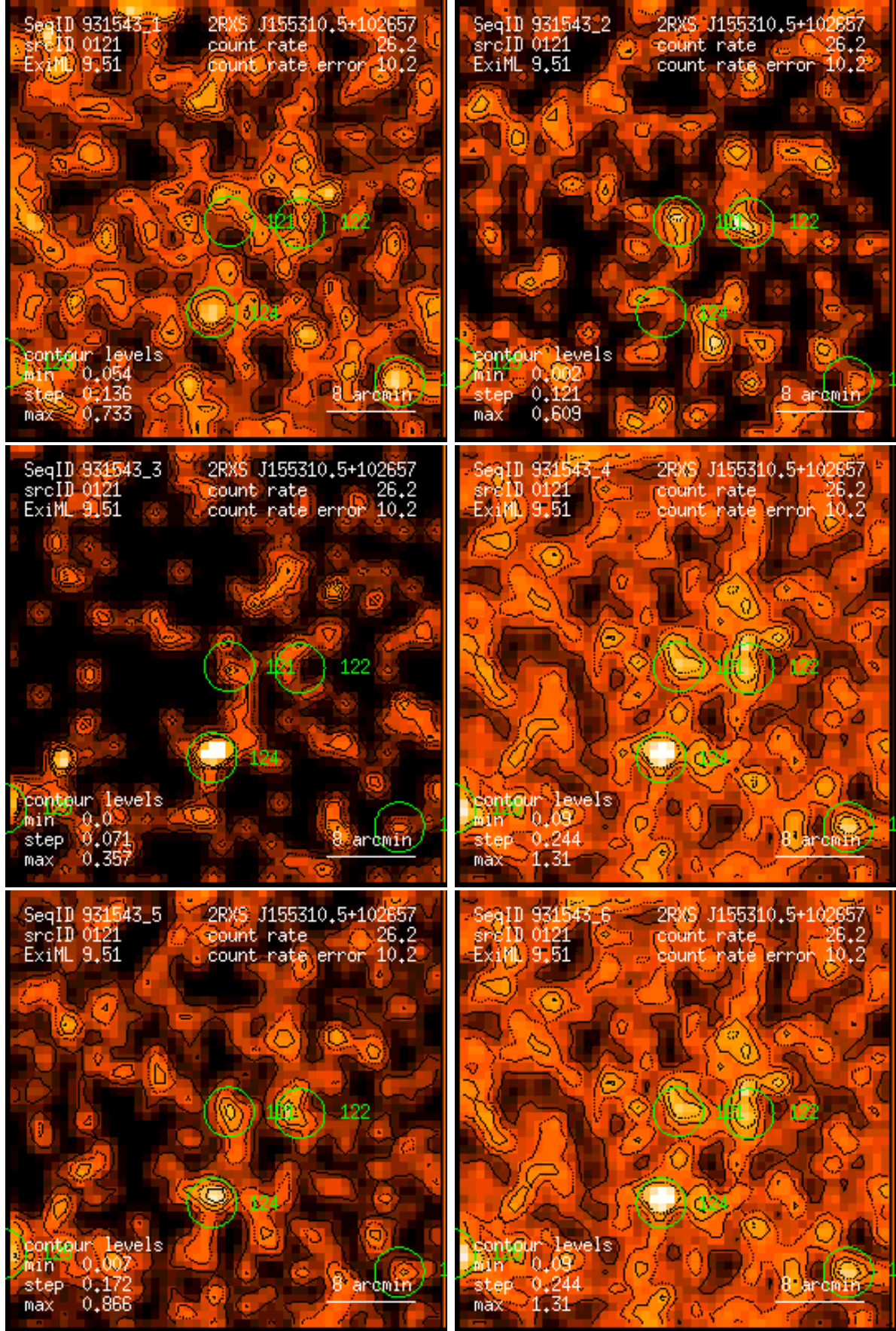
Figure 121: RASS 931543: detection 0121: band rate images, Gaussian filter: (1) PSPC channels 11 – 41, (2) 52 – 90, (3) 91 – 201, (4) 11 – 235, (5) 52 – 201, (6) 11 – 201. Broad band rates in counts/ks. Band rate contour levels in counts/ks/arcmin 2 .
