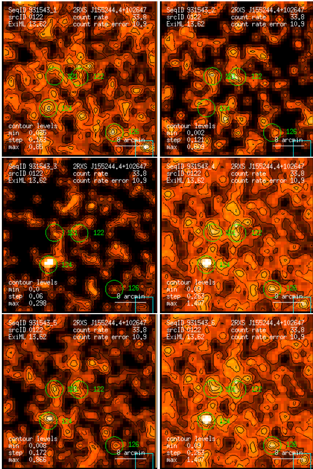
Figure 122: RASS 931543: detection 0122: band rate images, Gaussian filter: (1) PSPC channels 11 – 41, (2) 52 – 90, (3) 91 – 201, (4) 11 – 235, (5) 52 – 201, (6) 11 – 201. Broad band rates in counts/ks. Band rate contour levels in counts/ks/arcmin 2 .
