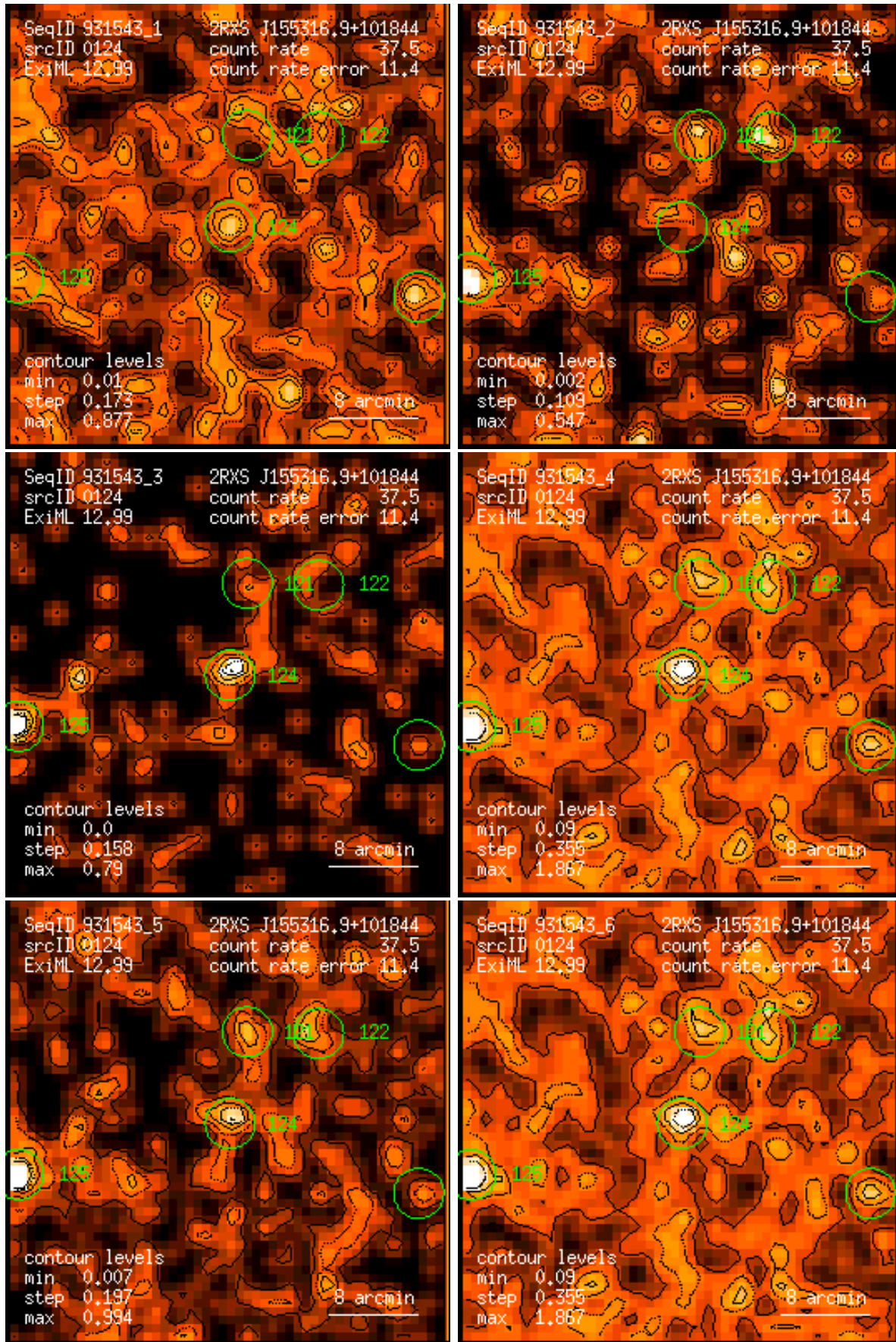
Figure 124: RASS 931543: detection 0124: band rate images, Gaussian filter: (1) PSPC channels 11 – 41, (2) 52 – 90, (3) 91 – 201, (4) 11 – 235, (5) 52 – 201, (6) 11 – 201. Broad band rates in counts/ks. Band rate contour levels in counts/ks/arcmin 2 .
