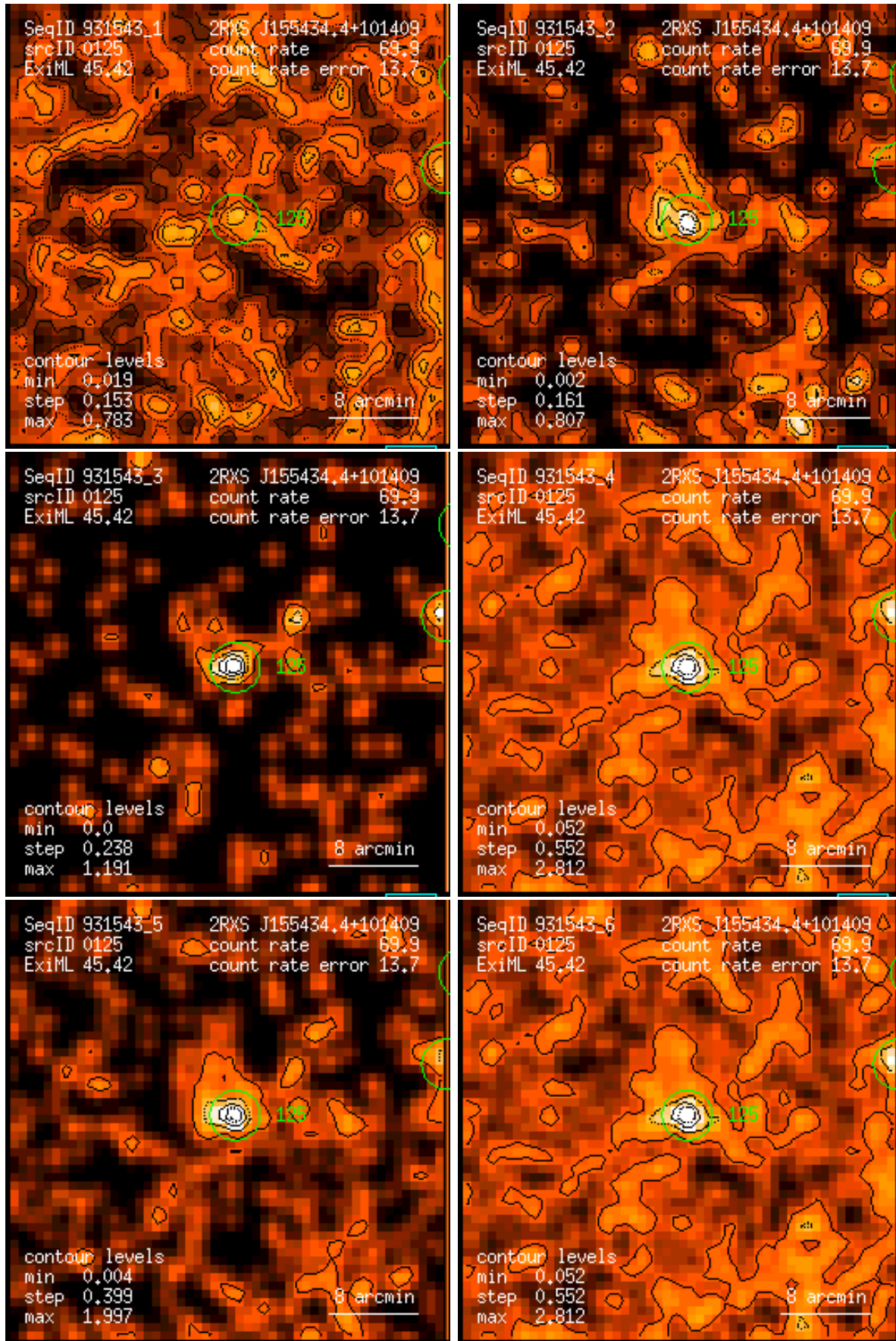
Figure 125: RASS 931543: detection 0125: band rate images, Gaussian filter: (1) PSPC channels 11 – 41, (2) 52 – 90, (3) 91 – 201, (4) 11 – 235, (5) 52 – 201, (6) 11 – 201. Broad band rates in counts/ks. Band rate contour levels in counts/ks/arcmin 2 .
