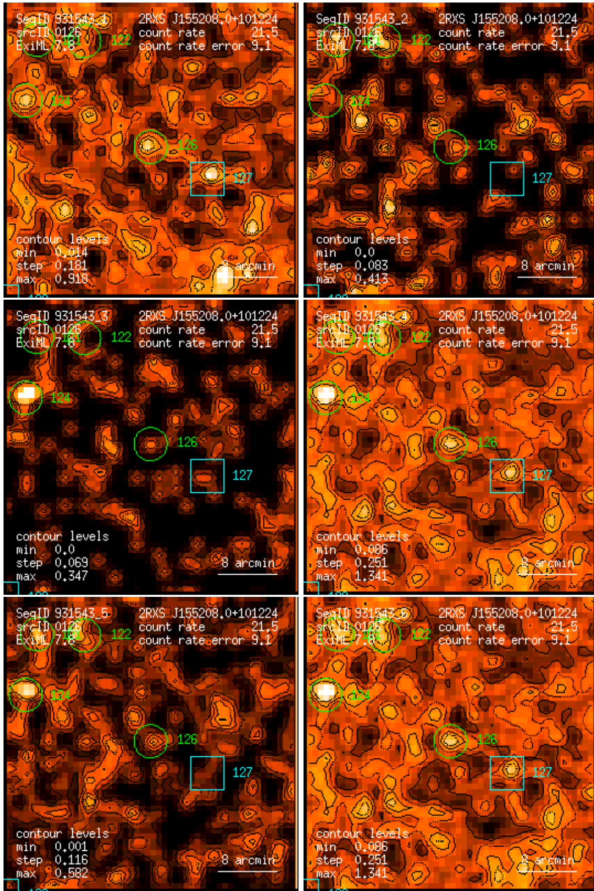
Figure 126: RASS 931543: detection 0126: band rate images, Gaussian filter: (1) PSPC channels 11 – 41, (2) 52 – 90, (3) 91 – 201, (4) 11 – 235, (5) 52 – 201, (6) 11 – 201. Broad band rates in counts/ks. Band rate contour levels in counts/ks/arcmin 2 .
