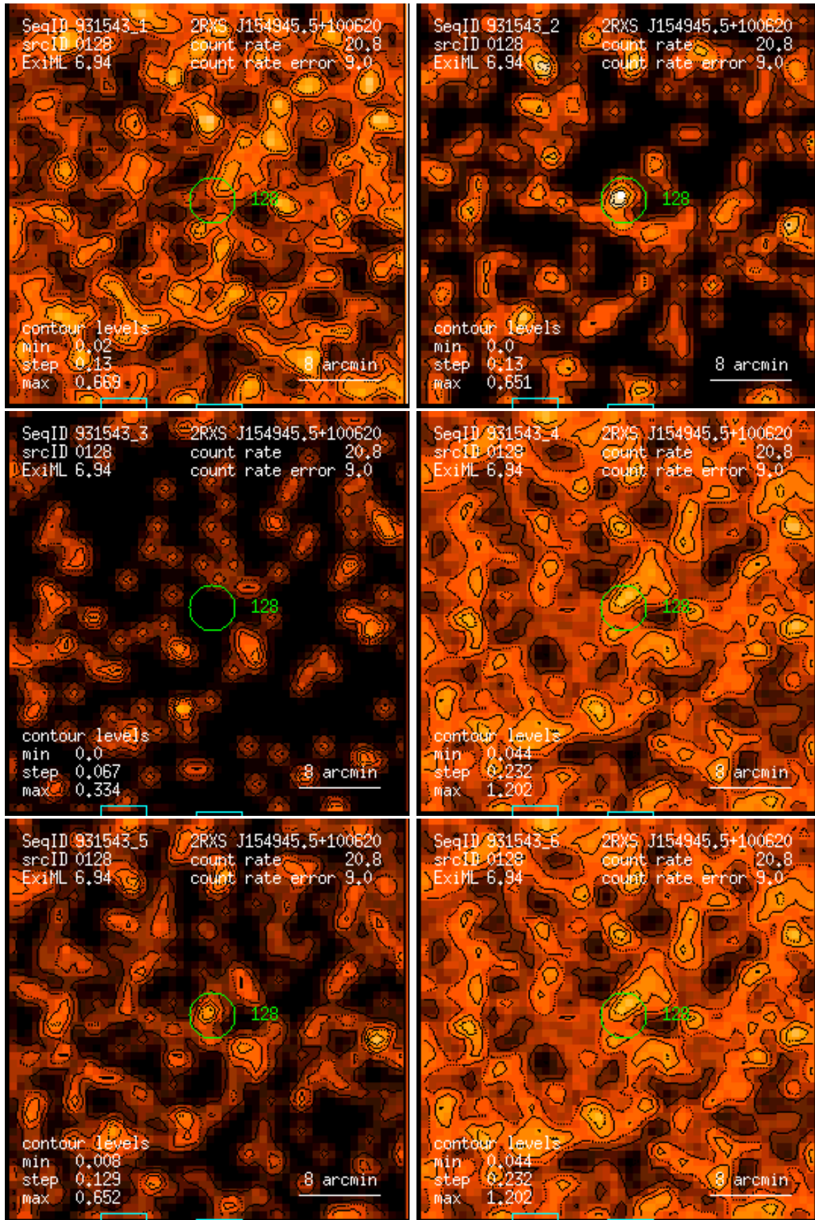
Figure 128: RASS 931543: detection 0128: band rate images, Gaussian filter: (1) PSPC channels 11 – 41, (2) 52 – 90, (3) 91 – 201, (4) 11 – 235, (5) 52 – 201, (6) 11 – 201. Broad band rates in counts/ks. Band rate contour levels in counts/ks/arcmin 2 .
