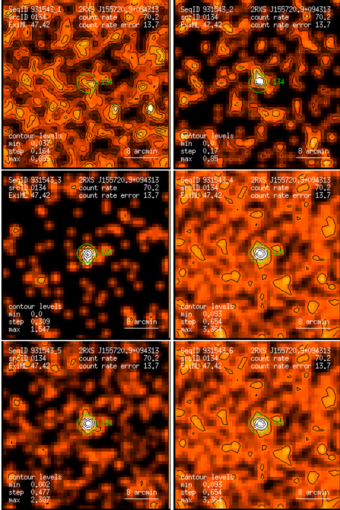
Figure 134: RASS 931543: detection 0134: band rate images, Gaussian filter: (1) PSPC channels 11 – 41, (2) 52 – 90, (3) 91 – 201, (4) 11 – 235, (5) 52 – 201, (6) 11 – 201. Broad band rates in counts/ks. Band rate contour levels in counts/ks/arcmin 2 .
